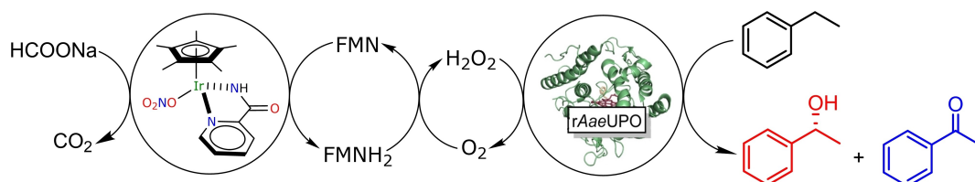
Scheme 2. Chemoenzymatic oxyfunctionalisation of ethylbenzene promoted by [Cp*Ir(pica)NO 3 ] and rAaeUPO catalytic tandem.
