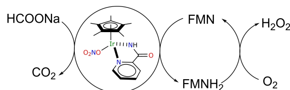
Scheme 1. In situ production of \text{H}_2\text{O}_2 by coupling the regeneration of FMNH 2 catalysed by [\text{Cp}^*\text{Ir}(\text{pica})\text{NO}_3] , using formate as hydride source, with the spontaneous reaction of FMNH 2 under aerobic conditions.
