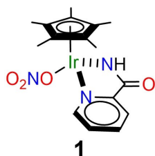
Figure 1. Sketch of [\text{Cp}^*\text{Ir}(\text{pica})\text{NO}_3] ( 1 ).
