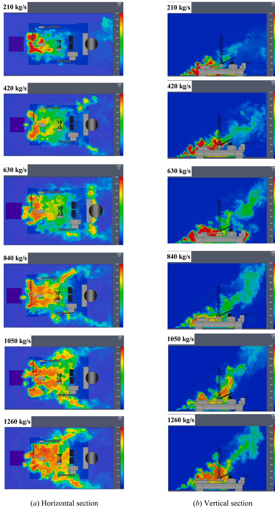
Fig. 12. Temperature field of steady fire under different gas release rates.
