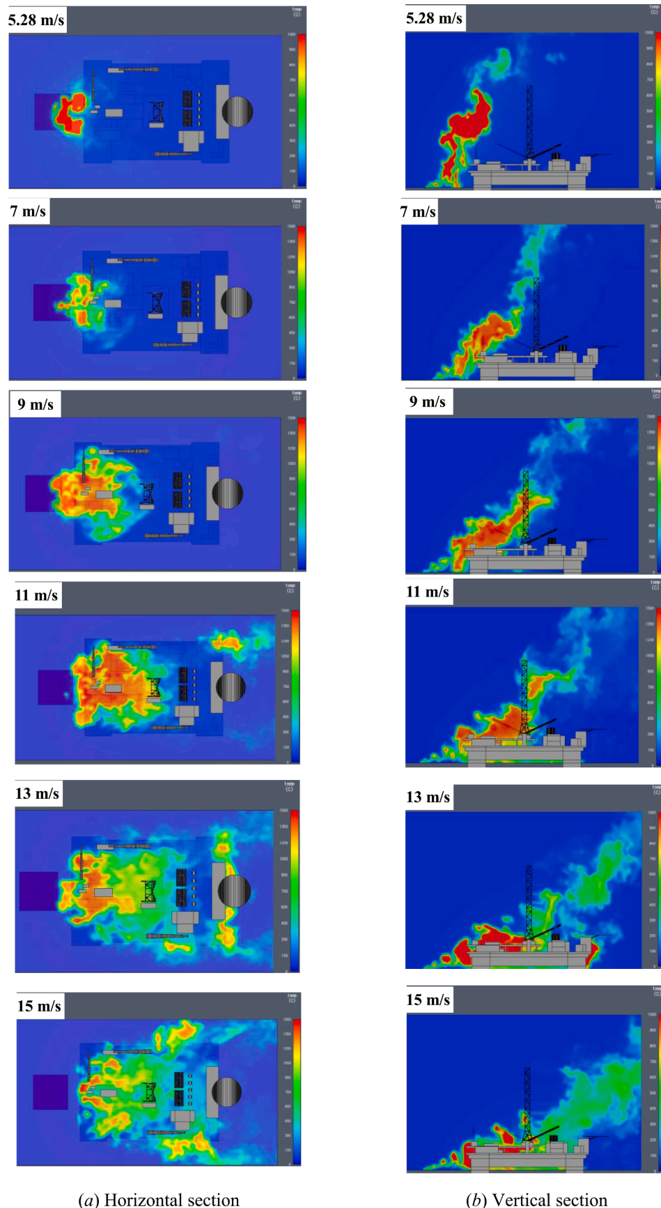
Fig. 9. Temperature field of steady fire under different wind speeds.
