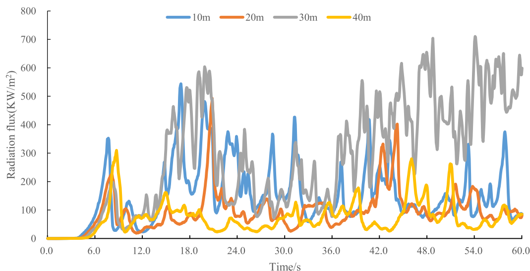
Fig. 16. Time-dependent profile of heat radiation flux with of distance between release and platform.
