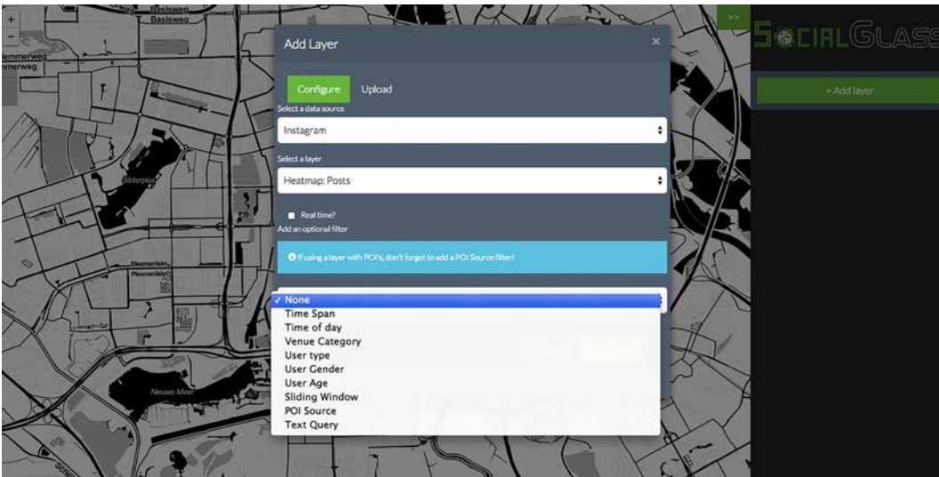
FIGURE 34 Data filters.
