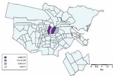
Local Moran's I – FDR adjusted p -values
