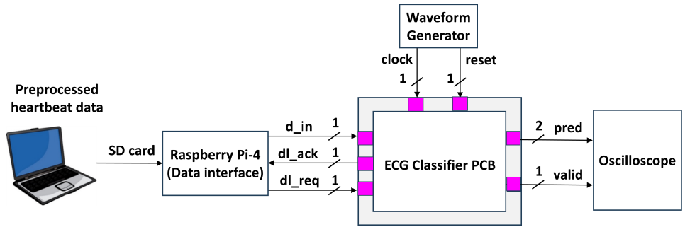
Figure 8.10: Testbench for prototype evaluation.
