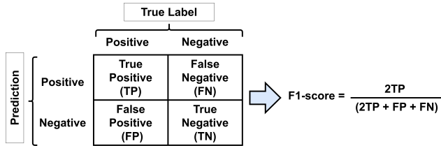
Figure 4.5: F1-score calculation from confusion matrix representation.
