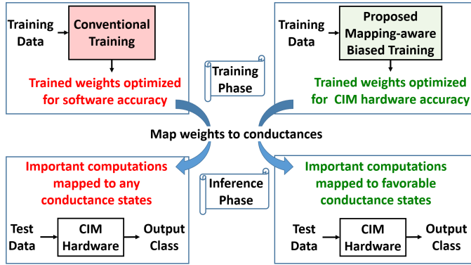
Figure 5.1: Overview of the conventional and proposed training methodologies.
