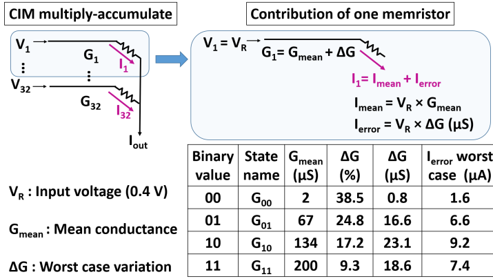
Figure 5.2: Favorable conductance states analysis for a 2-bit memristor (four conductance states). The used conductance variation data is obtained from [147].
