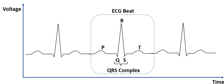
Figure 3.1: Illustration of 'PQRST' cycle for an ECG beat, where P: atrial contraction, Q: interventricular septum contraction, R: ventricular contraction (main mass), S: ventricular contraction (at heart's base), and T: ventricular relaxation. Atrial relaxation is obscured by QRS complex.
