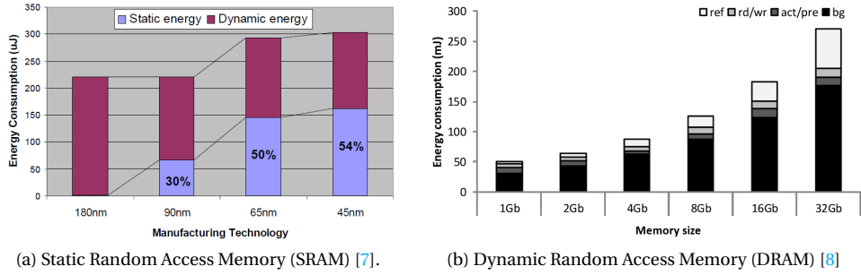
Figure 1.4: Energy consumption breakdown for conventional memory technologies. In subfigure (b), rf: refresh energy, rd/wr: read/write energy, act/pre: activate/precharge energy, and bg: background energy.
