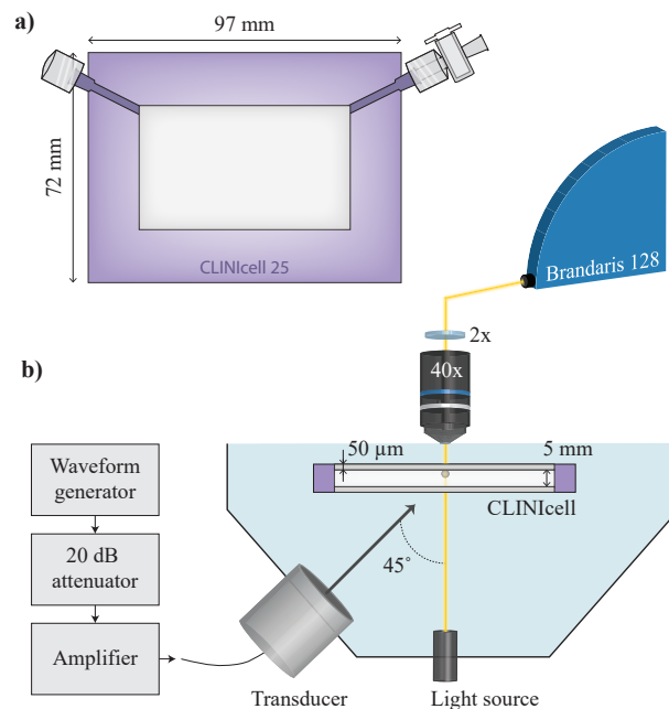
Fig. 1. a) Sketch of a CLINiCell with a 25 cm 2 cell culture area. b) Schematic representation (not drawn to scale) of the experimental setup to study microbubble oscillation upon insonification using the Brandaris 128 ultra-high speed camera. The two parallel membranes of the CLINiCell each have a thickness of 50 \mu\text{m} . The microscope was equipped with a 40 \times water immersion objective and a 2 \times lens (Olympus, Tokyo, Japan). The insonification scheme was generated by a waveform generator (Tabor 8026, Tabor Electronics, Tel Hanan, Israel), connected to a 20 dB attenuator (Mini-Circuits, Brooklyn, NY, USA) and a broadband amplifier (ENI A-500, Electronics & Innovation, Rochester, NY, USA).
