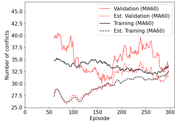
Figure 4. Evolution of the estimated number of conflicts during testing and validation of the CEN.
