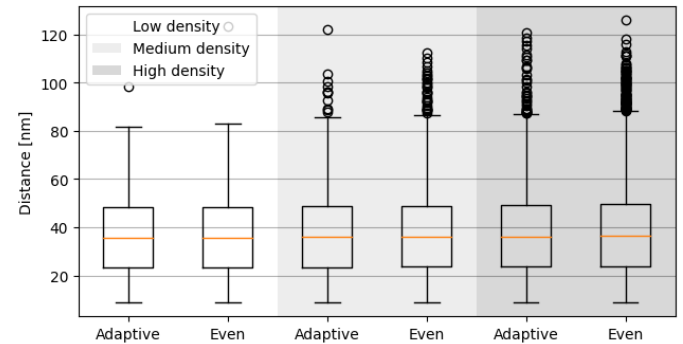
Figure 14. Total distance travelled resulting from employing the heading ranges per layer output by the supervised learning model (Adaptive) and an even heading range distribution per layer (Even), for all traffic densities with conflict resolution.
