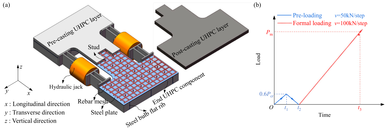
Fig. 4. (a) Test setup and (b) loading protocol.
