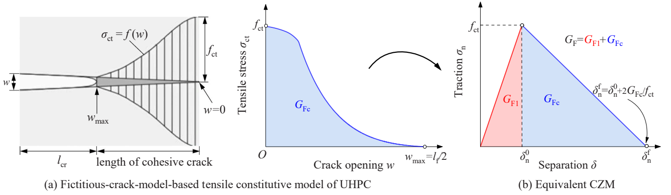
Fig. 20. Equivalent cohesive zone model from the tensile constitutive model of UHPC.
