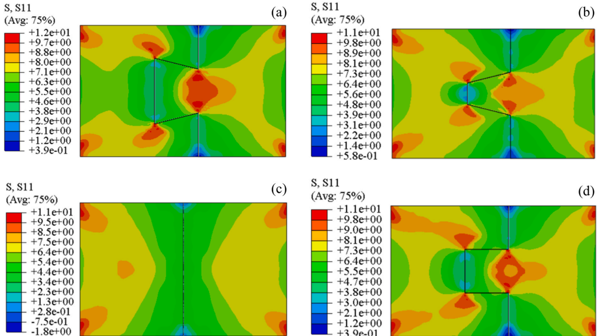
Fig. 29. Longitudinal normal stress distribution of the UHPC layer at P = 2500 kN: (a) \alpha = 14^\circ ; (b) \alpha = -14^\circ ; (c) \alpha = 0^\circ ; and (d) \alpha = 90^\circ .
