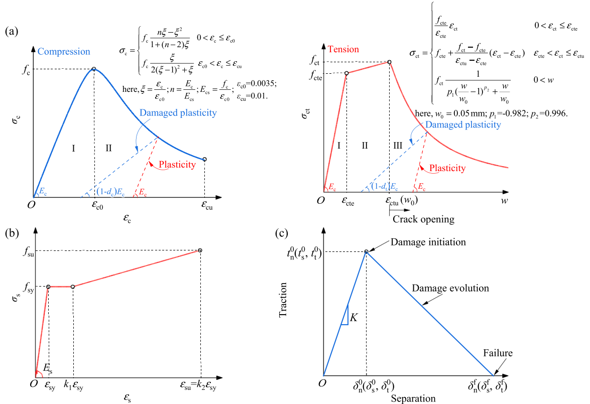
Fig. 10. Material constitutive models: (a) UHPC; (b) steel; and (c) traction-separation law for cohesive zone model.
