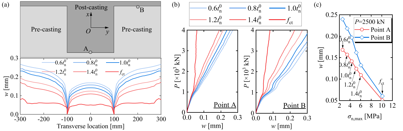
Fig. 21. Influence of bond strength on crack opening displacement at the interface: (a) crack opening distribution under P = 2500 kN; (b) axial load-crack opening displacement response; and (c) crack opening displacement-bond strength relation.
