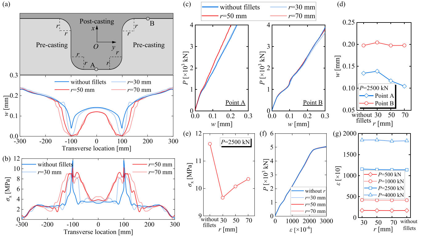
Fig. 30. Influence of fillet radius on crack opening displacement at the interface: (a) crack opening distribution under P = 2500 kN; (b) longitudinal normal stress distribution at the interface under P = 2500 kN; (c) axial load-crack opening displacement response; (d) crack opening displacement-fillet radius relation; (e) longitudinal normal stress-fillet radius relation at the interface intersection; (f) axial load-average rebar strain response; and (g) average rebar strain-fillet radius relation.
