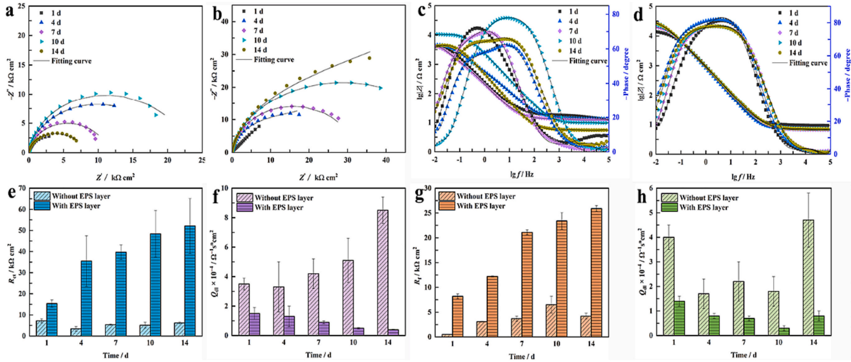
Fig. 6. Impedance spectrum and fitting parameters of coupons (a, c) without and (b, d) with EPS layer exposed to N. dassonvillei inoculated medium: (e) R_{ct} , (f) Q_{dl} , (g) R_t , (h) Q_r .
