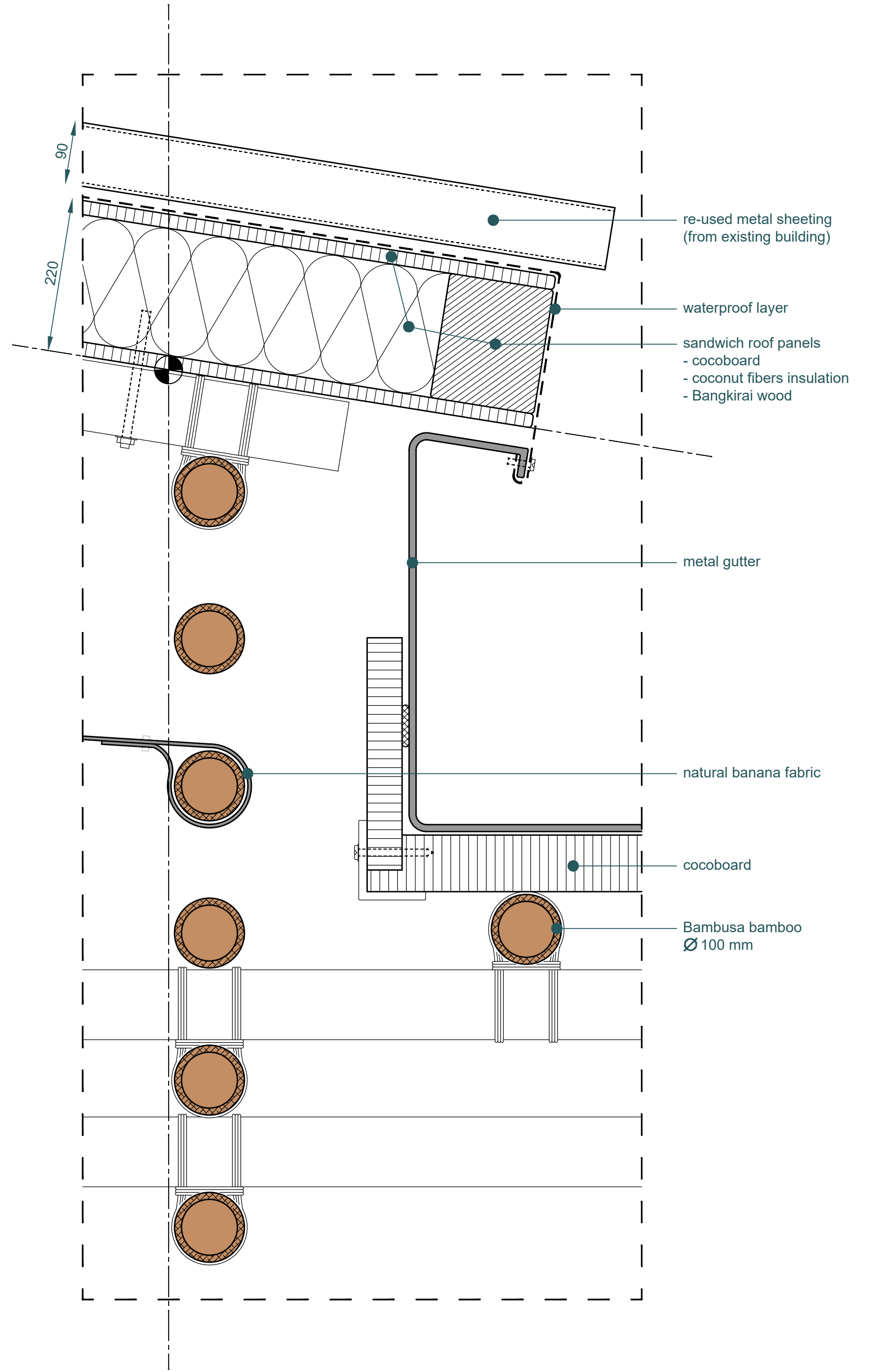
DETAIL 1 | 1:5
