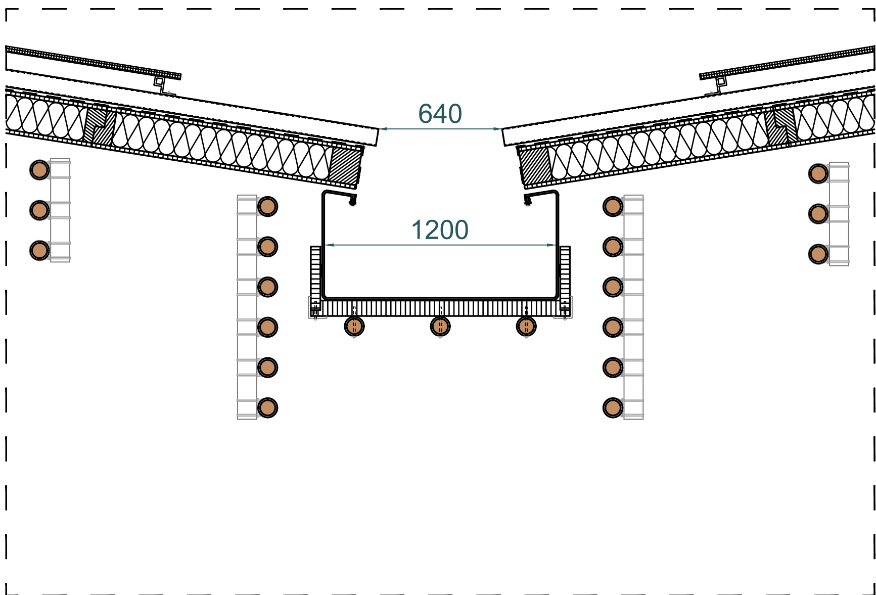
VERTICAL SECTIONS | 1:20
