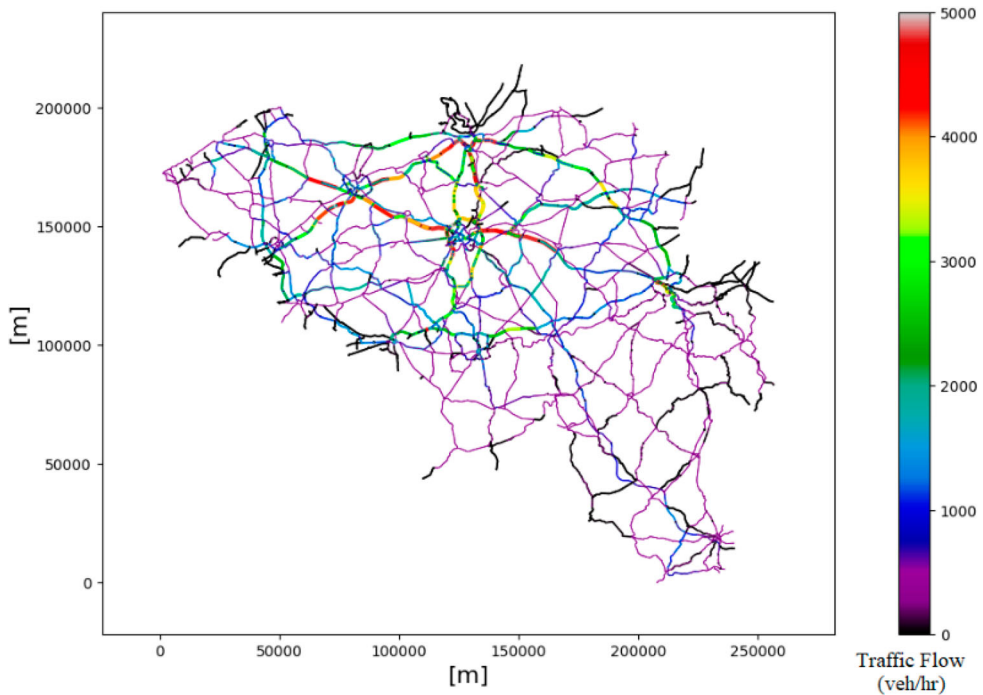
Figure 4. Simulated peak hour traffic flow of the Belgium road network.
