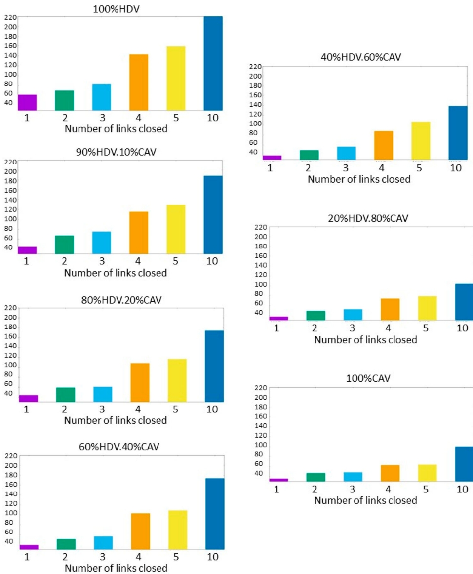
Figure 6. Resilience Loss for all scenarios (Veh. Min x1000).
