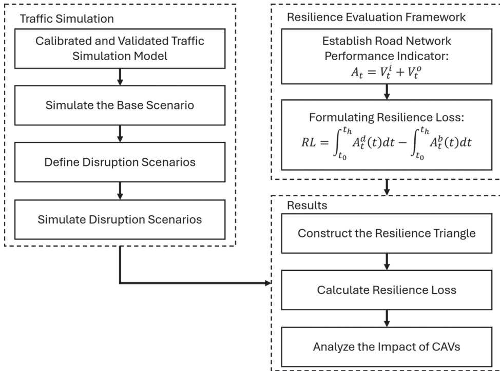
Figure 3. Road network resilience evaluation methodology.
