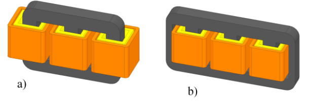
Fig. 2. Transformer types; a) core-type, b) shell-type
