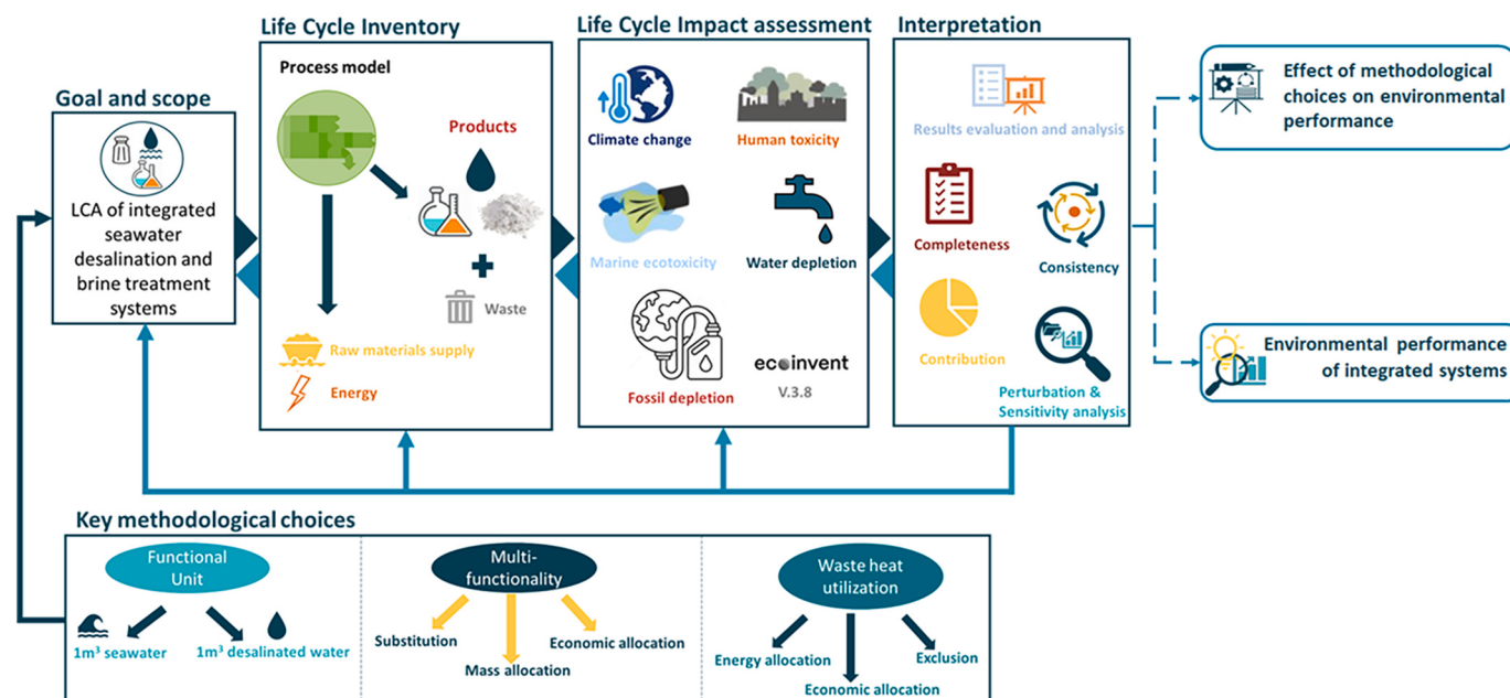
Fig. 1. Life Cycle Assessment (LCA) for integrated seawater desalination and brine treatment systems: an overview of methodological approach, related steps and key choices. Key methodological choices related to the functional unit, multifunctionality and the inclusion of waste heat utilization in the background system made in the goal and scope. Light blue line arrows denote feedback loops in the methodological steps and revisions in the methodological choices.
