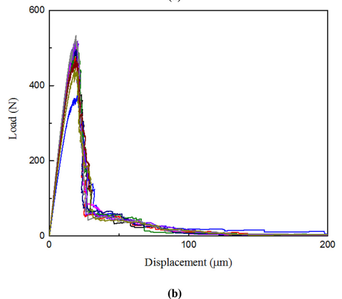
Fig. 13. Simulated load-displacement curve of the digital specimens with size of (a) 0.1 mm and (b) 5 mm.
