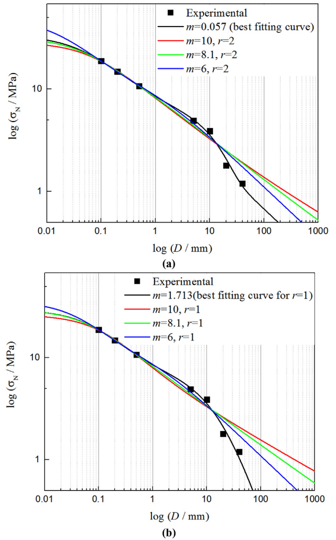
Fig. 11. Fits of Bažant's ESSET with different m : (a) r = 2 ; (b) r = 1 .
