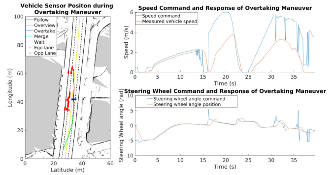
Fig. 27. Vehicle and obstacle positions, vehicle speed, and steering wheel angle plots for experiment scenario 3.
