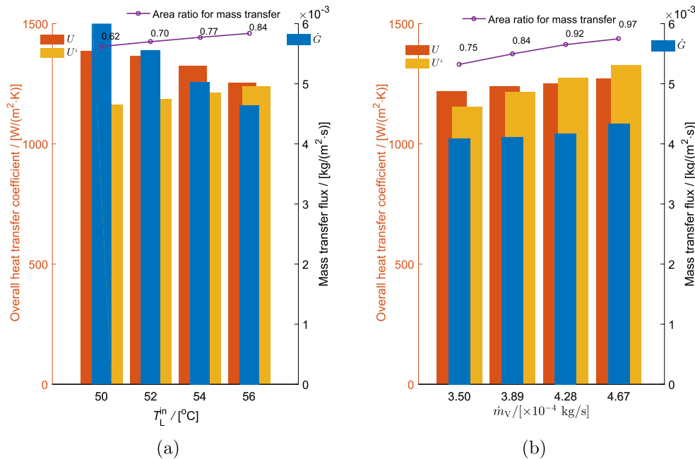
Fig. 15. Sensitivity analysis of (a) solution inlet temperature and (b) vapor flow rate on the overall heat and mass transfer performance of \text{NH}_3 's absorption into \text{NH}_3 /[emim][ \text{Tf}_2\text{N} ] solution.
