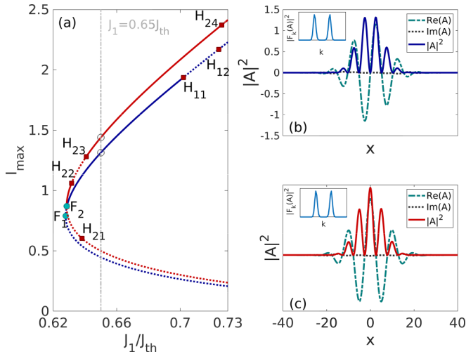
FIG. 7. (a) Branches of one-dimensional tilted HG modes \Gamma_0 (red) and \Psi_0 (blue) of Eq. (25) as a function of the normalized gain bias J_1/J_{th} . The mode \Gamma_0 is stable (solid line) between the fold F_2 (cyan circle) and the AH point H_{22} as well as between AH points H_{23} and H_{24} (red squares), respectively. The mode \Psi_0 gains the stability at the fold F_1 and remains stable up to the AH bifurcation point H_{11} . (b), (c) Exemplary profiles of \Gamma_0 and \Psi_0 for J_1 = 0.65J_{th} (gray dashed line). Real (turquoise, dashed), imaginary (black, dotted), and intensity fields (blue, red, solid), respectively, are presented. Parameters are \alpha_1 = 1.5 , \alpha_2 = 0.5 , J_2 = -0.06 , \hat{s} = 15 , \kappa = 0.035 , d_f = 10^{-4} , b = 0.78 , c = 4.97 \times 10^{-4} , s = 1.0 .
