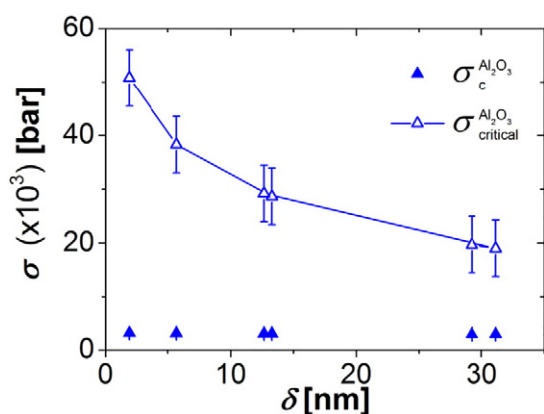
Fig. 4. Tensile stress ( \sigma_c^{\text{Al}_2\text{O}_3} ) exerted on the alumina-coated samples (blue symbols) and critical tensile stress ( \sigma_{\text{critical}}^{\text{Al}_2\text{O}_3} ) of the alumina before breaking (open symbols) for the different film thickness. The error bars represent the uncertainty in the calculation of the tensile stresses.
