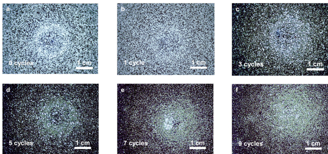
Fig. 12. Reverse Impact test, performed over the painted panels with 0, 1, 3, 5, 7 and 9 cycles. The thickness of the paint was around 50 μm in all the samples. The contrast and brightness of the pictures were modified for a better visualization of the cracks.
