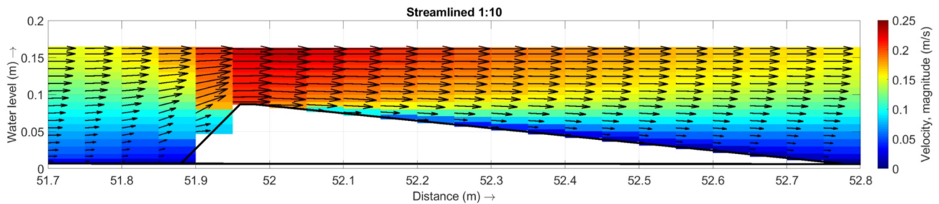
Figure 11. Flow velocity contours and vectors over a groyne at y = 2.25 m after streamlining the downstream face to 1V:10H (case h160).
