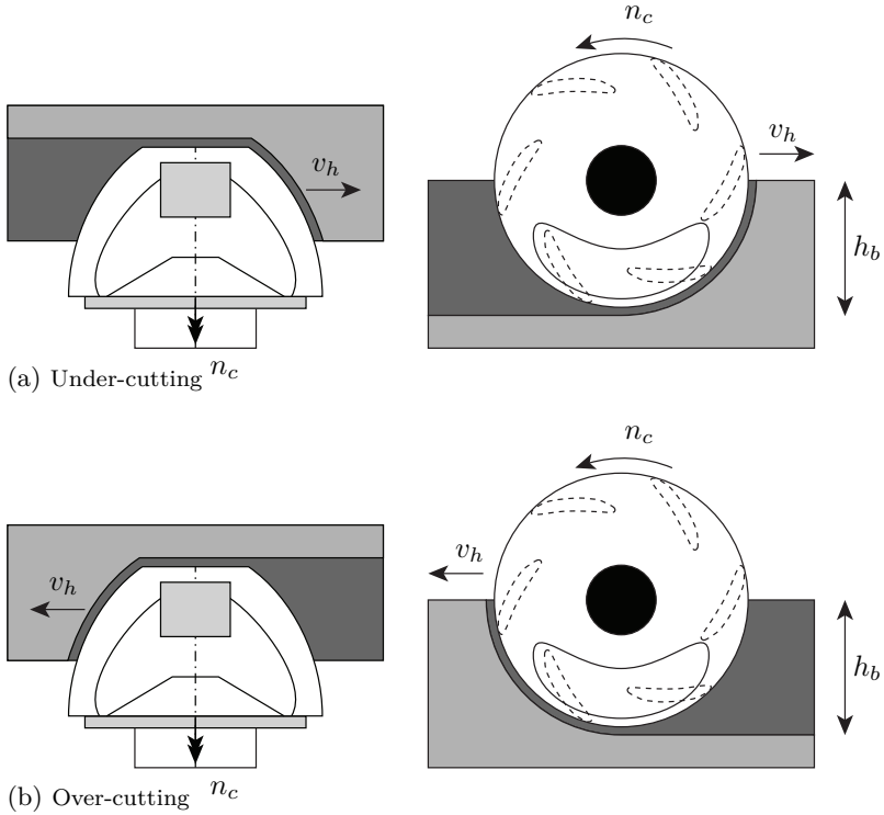
Figure 2.4: Schematic view of under- and over-cutting. It shows the cross-section along the axis (left) and perpendicular to the axis (right) of the two different cutting method. The light-grey indicates the bank, which is still to be cut. The dark grey indicates the breach. It also shows the hauling velocity ( v_h ), rotational velocity ( n_c ) and breach height ( h_b ) (adapted after Den Burger (2003)).
