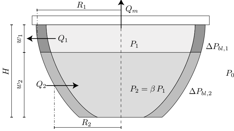
Figure 4.8: Pressures and flows in the segments.
