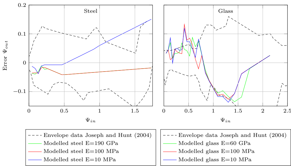
Figure 7.8: Errors in the simulation of an obliquely colliding 12.7 mm sphere, where the envelope is defined as the difference of the data with the trend line.
