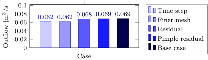
Figure 5.12: Sensitivity analysis based on the out-flowing flux for the different cases.
