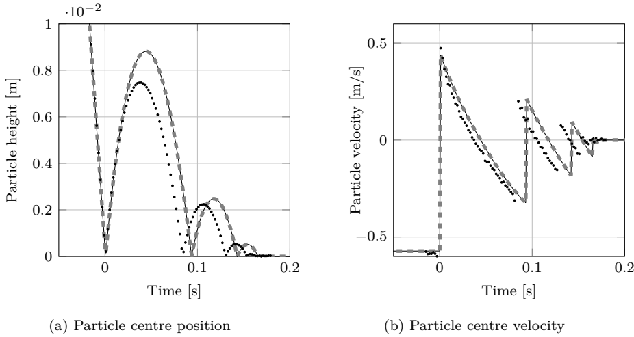
Figure 7.1: Simulation of a falling 3 mm steel particle in viscous oil compared with the experimental results of Gondret et al. (2002) ( \circ ). The simulations are executed for two particle diameters over cell size ratios. d_p/\Delta x = 0.1 (—) and d_p/\Delta x = 5 (---).
