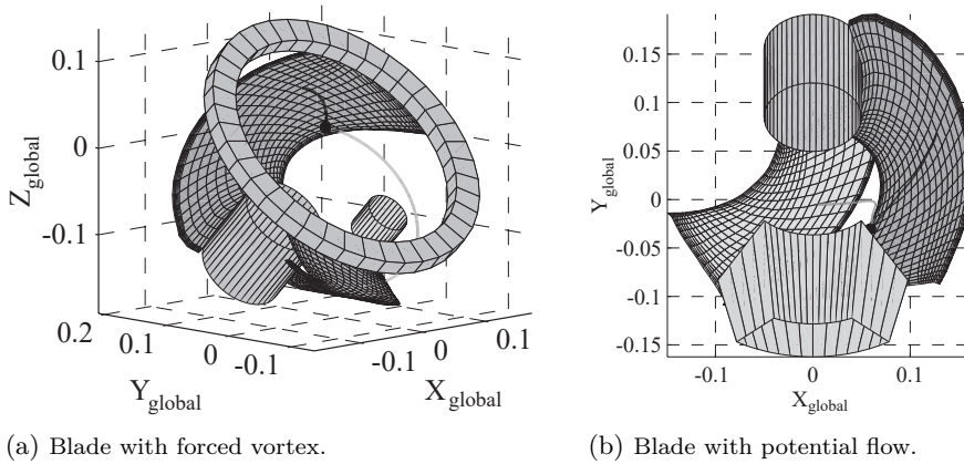
Figure 2.15: Simulated particle transported over the blade towards the suction mouth. The black dot represents the position at the end of the simulation (Den Burger, 2003).
