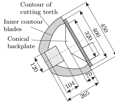
Figure 2.11: Dimensions of the cutter head used for the gravel cutting experiments in mm (Den Burger, 2003).
