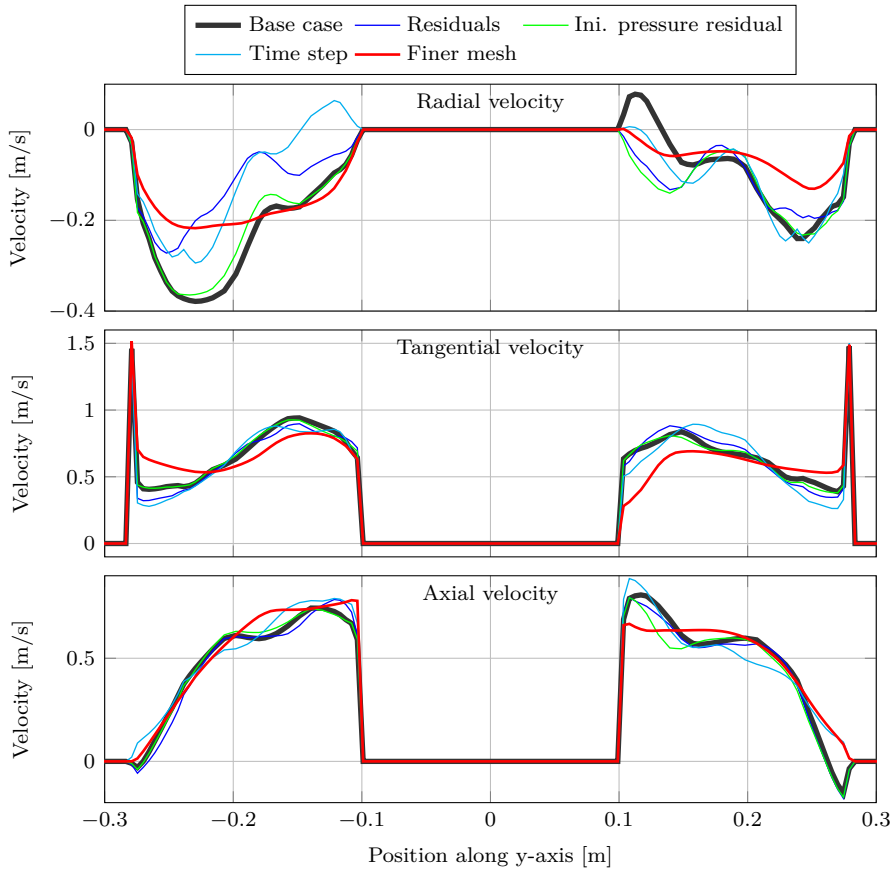
Figure 5.11: Line plots of the velocity components in the cutter head with uniform suction at z=-0.035\text{m} along the y-axis. Positive radial velocities indicate outward flow, positive tangential velocities are in the rotational direction and positive axial velocities are from the hub to the suction mouth.
