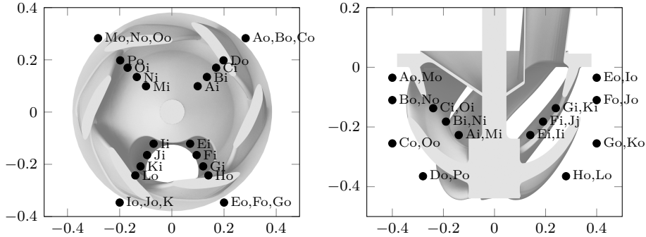
Figure B.1: Measurement locations in and around the cutter a backplate and suction mouth.
