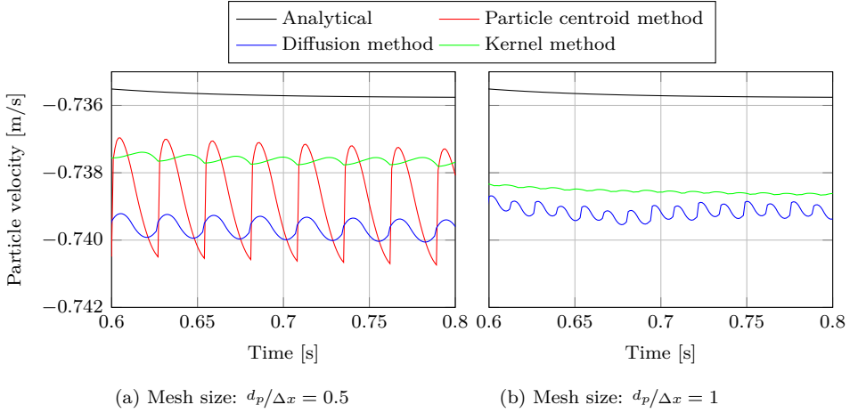
Figure 6.5: Particle velocity oscillations for the three simulation methods for mesh size d_p/\Delta x = 0.5 and d_p/\Delta x = 1 .
