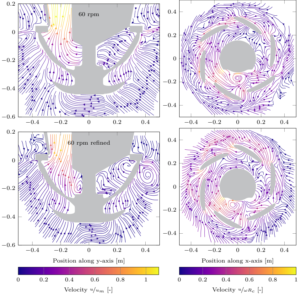
Figure 5.20: Instantaneous streamlines of the simulation results for 2 different numerical settings after 14 rotations. Top: base case and bottom: 25% mesh refinement. The colours show the in-plane velocity magnitudes. The left plots show the yz-plane at x=0 . The right plots show the azimuthal plane (xy-plane) at z=-0.035
