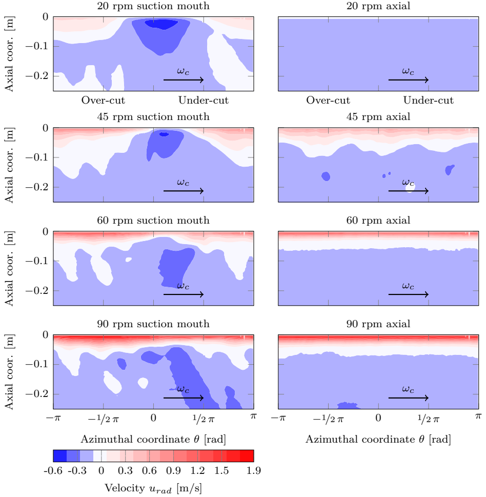
Figure 8.2: Time averaged radial outflow velocities around the cutter head. The suction mouth is located at \theta = 0 and the rotational velocity is from left to right. The velocities have been averaged over 1 rotation of the cutter head. Only the top part of the cutter head is visualised.
