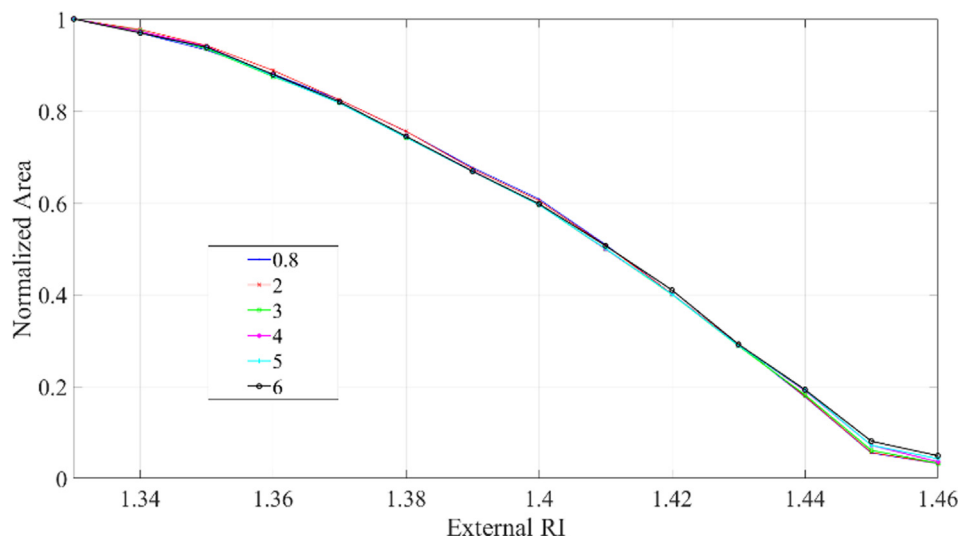
Fig. 14. Correlation ERI-Normalized Area performed with several \alpha values for 5° tilted FBG sensor written in thin-OF.
