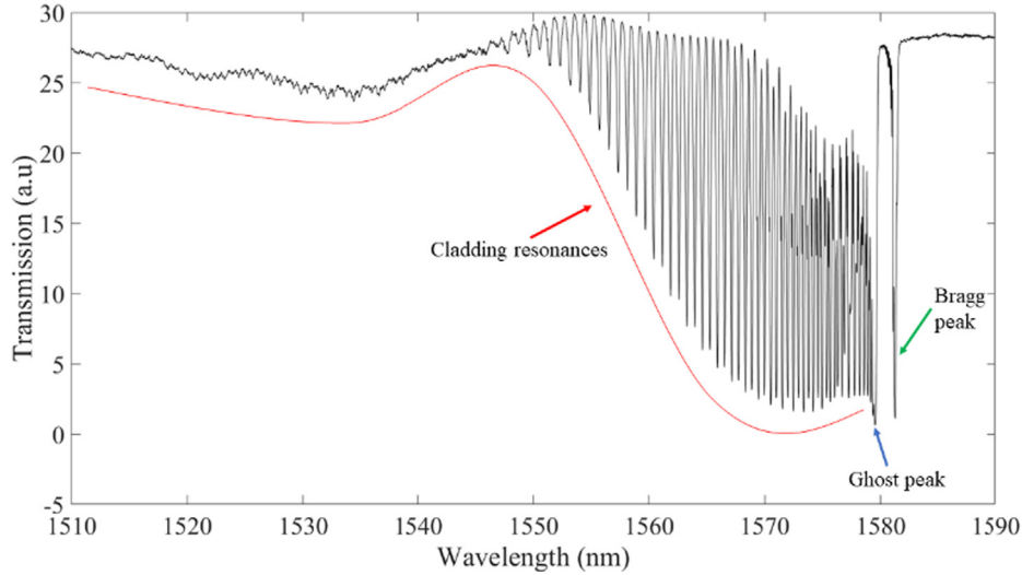
Fig. 2. Bragg, Ghost and cladding resonances in the transmission spectrum of a 5° tilted FBG written in Fibercore SM1500(9/125)P OF.
