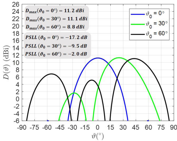
FIGURE 16. Scanned pattern ( \varphi = 0^\circ ) of the subarray Type 4c with P_{4c,n} = 3 , \lambda/2 -grid elements and amplitude of B_{n(4c)} = [0.9; 0.95; 1] for p_{4c,n} = 1, 2 , and 3 . The patterns are obtained for positive scanning angles, \vartheta_0 = 0^\circ, 30^\circ , and 60^\circ .
