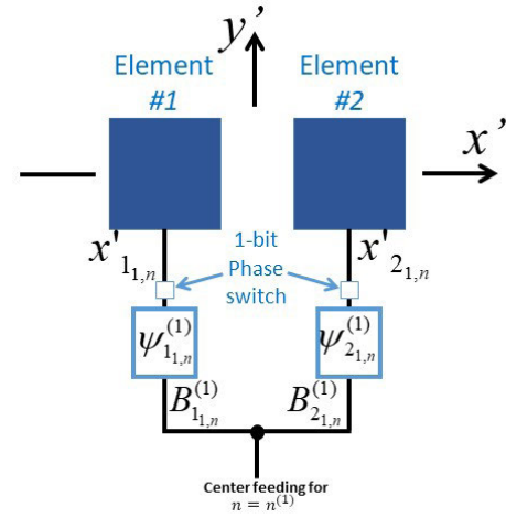
FIGURE 2. Two-element in-line subarray configuration (Subarray Type 1). Subarray elements are located at x'_{p_{1,n}} and fed with complex excitations determined by amplitudes B_{p_{1,n}}^{(1)} and phases \psi_{p_{1,n}}^{(1)} .
