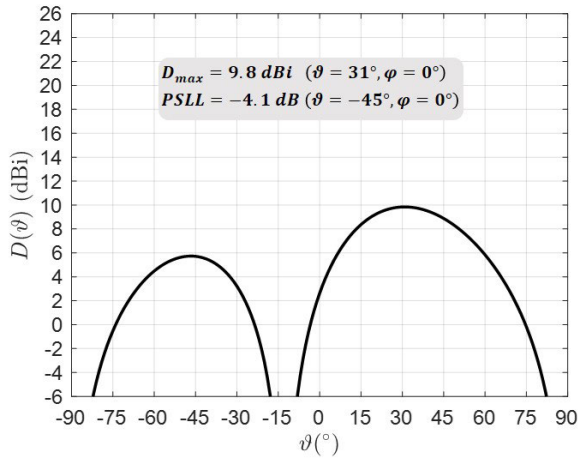
FIGURE 9. Pattern ( \varphi = 0^\circ ) of the subarray Type 1 (2 elements), with B_{1,n}^{(1)} = B_{2,n}^{(1)} = 0.7 , \psi_{1,n}^{(1)} = +70^\circ , \psi_{2,n}^{(1)} = -70^\circ , and \lambda/2 -grid elements. This subarray pattern is for positive scan angles application, while for the negative scan angles the pattern is just its mirror around broadside.
