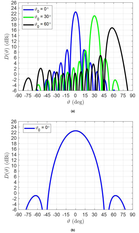
FIGURE 22. Array patterns of the subarray Type 4a ( P_{4a,n} = 13 , uniform amplitudes, and stretched spacing) integrated with subarray Type 3a with amplitude distribution of B_{p_{3a,n}}^{(3a)} = [0.505; 0.7; 0.505] for p_{3a,n} = 1, 2 , and 3. (a) azimuth pattern while scanning from broadside up to \vartheta_0 = 60^\circ ; (b) elevation pattern for broadside scanning.
