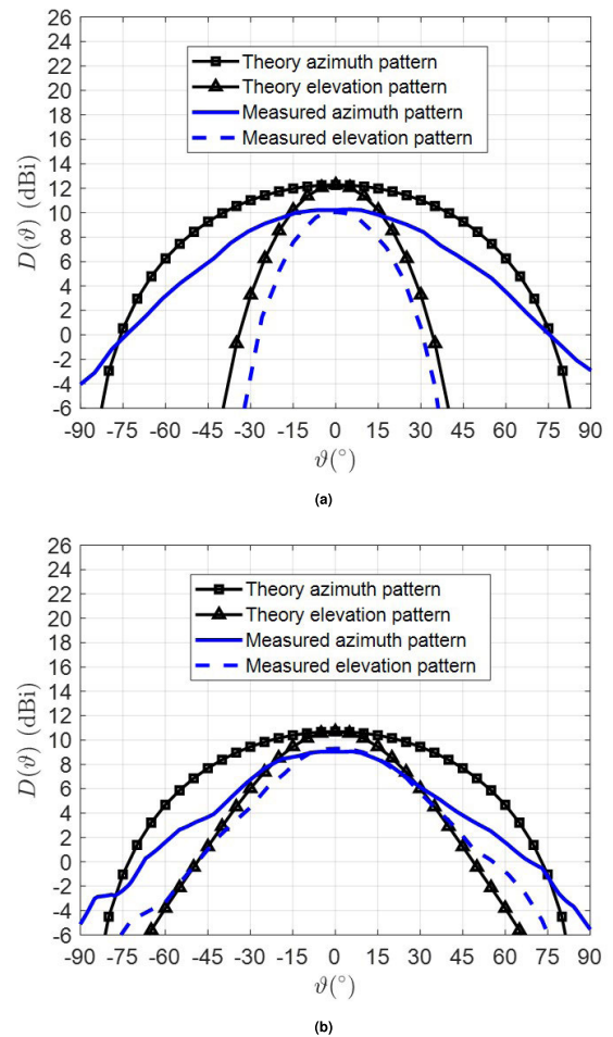
FIGURE 20. The magnitude pattern comparison between measurement and theoretical calculation results in azimuth and elevation plane. (a) Subarray Type 3a; (b) Subarray Type 3b.
