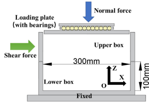
(b) Schematic diagram
