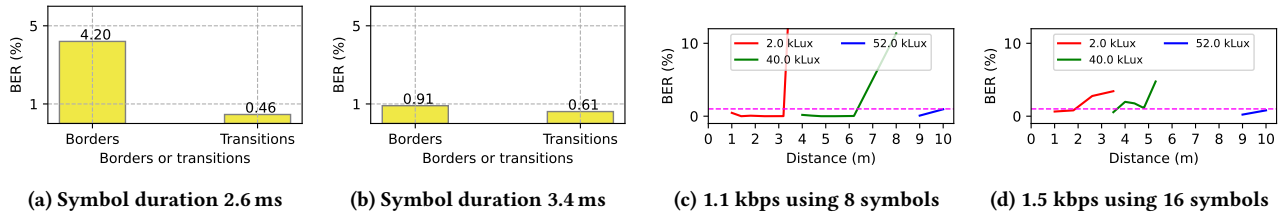
Figure 11: Comparison between using transitions versus borders (a) and (b), and BER performance at different distances (c) and (d).
