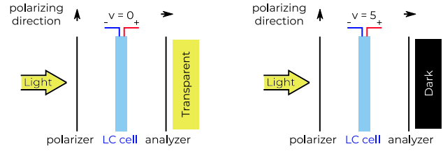
Figure 2: LC Operation. The LC cell is placed between two perpendicular polarizing sheets. If v = 0V , the light is rotated and passes the analyzer; if v = 5V , the light is blocked.
