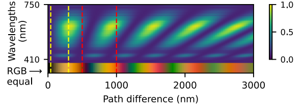
Figure 3: Modeled impact of path difference on flashlight spectrum per wavelength. The color on the bottom shows the combined effect of the wavelengths in the column above.
