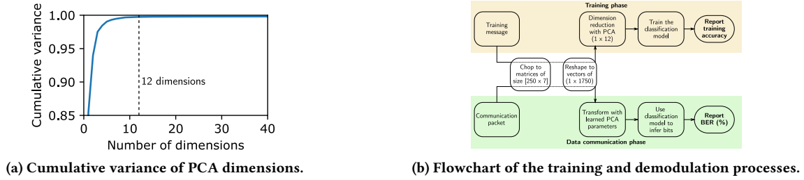
Figure 9: Cumulative variance as a function of PCA dimensions (a), and the system flowchart (b).
