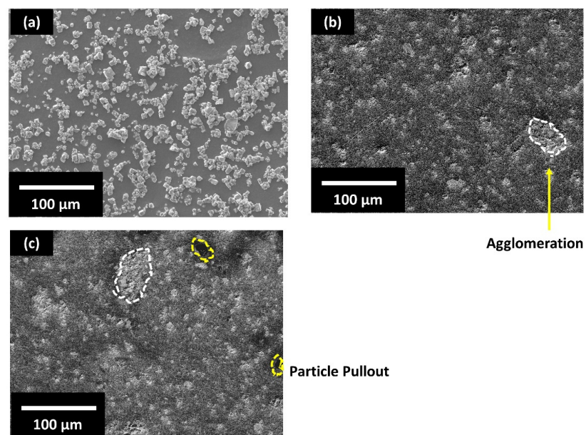
Figure 2. Scanning electron microscopy (SEM) image of: (a): KNLN ( \text{K}_{0.485}\text{Na}_{0.485}\text{La}_{0.03}\text{NbO}_3 ) powder; (b) horizontal cross section of the filament containing polylactic acid (PLA)-10 vol.% KNLN composite; (c) vertical cross section of the filament of PLA-10 vol.% KNLN composite (horizontal); white circles indicate agglomeration while yellow circles indicate particle pull-out.
