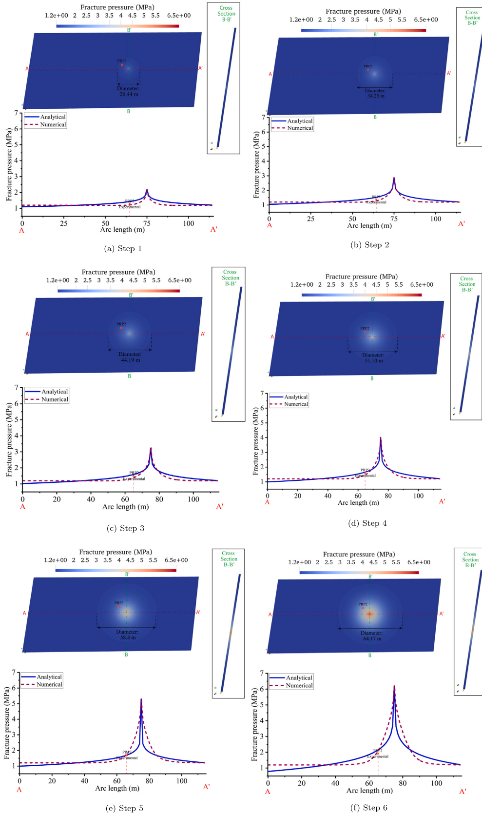
Fig. 10. Fracture pressure at different steps; (a) Step 1 : Injection pressure 2.33 MPa; flow rate 1.82 l/min; time 680 s, (b) Step 2: Injection pressure 3.07 MPa; flow rate 3.26 l/min; time 1260 s, (c) Step 3: Injection pressure 3.51 MPa; flow rate 4.3 l/min; time 1720 s, (d) Step 4: Injection pressure 4.27 MPa; flow rate 6.57 l/min; time 2080 s (e) Step 5: Injection pressure 5.37 MPa; flow rate 15.00 l/min; time 2730 s, (f) Step 6: Injection pressure 6.45 MPa; flow rate 25.00 l/min; time 3000 s.
