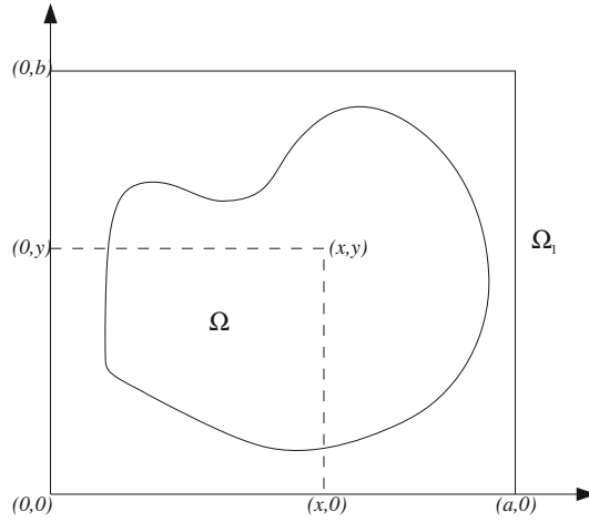
Figure 1.4: 2-dimensional region.
