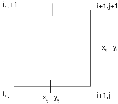
Figure 4.9: Cell in the \xi - \eta -plane with natural place of coordinate derivatives.
