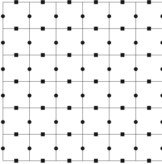
Figure 4.14: Staggered grid.
