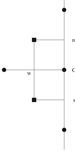
Figure 4.16: Half volume at natural boundary.
