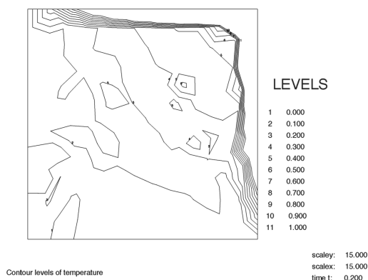
Figure 6.1: Contour lines of the numerical solution to the heat equation with \Delta t = 0.1 as obtained by the use of the Forward (explicit) Euler method (unstable solution).
