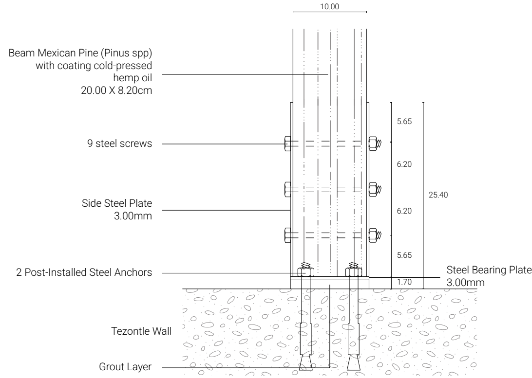
Detail from Column to Foundation
