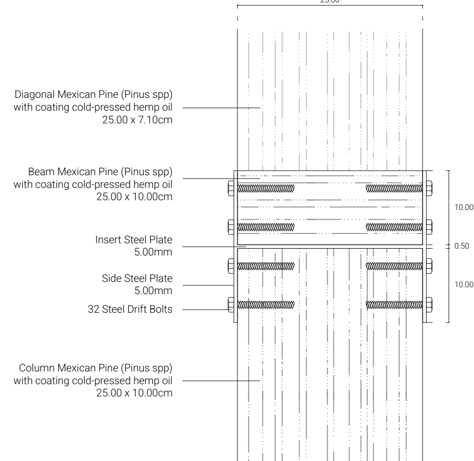
Detail from Column to Beam
