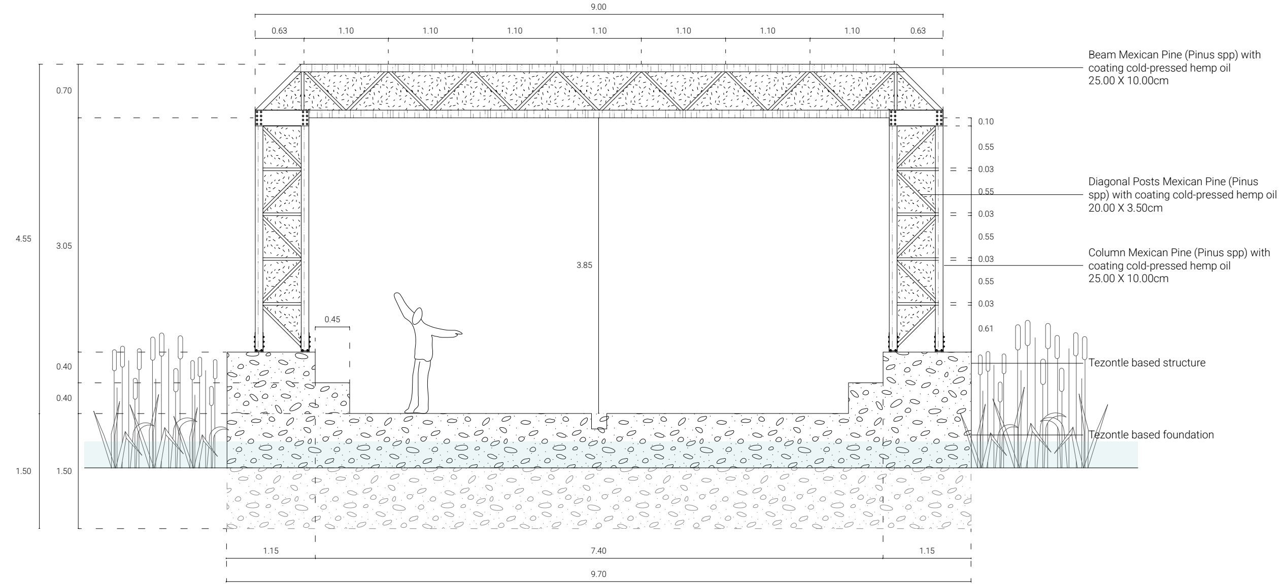
Section 2 Event Plaza
