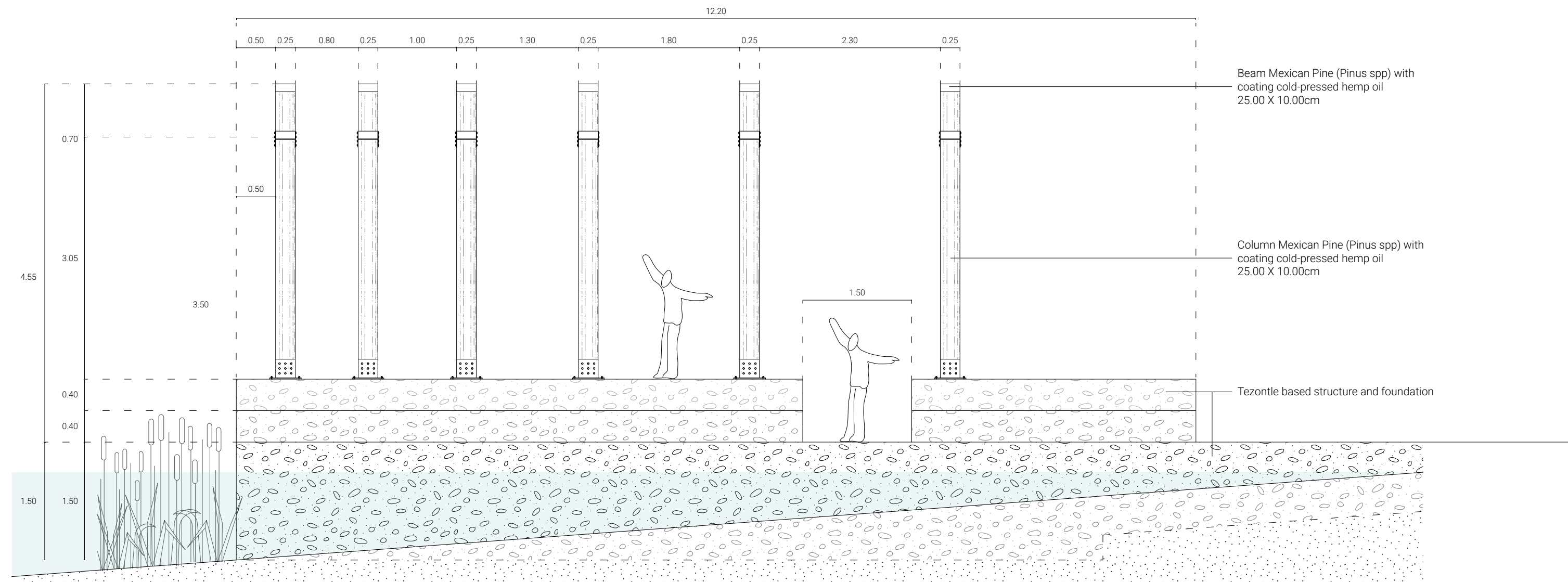
Section 1 Event Plaza
