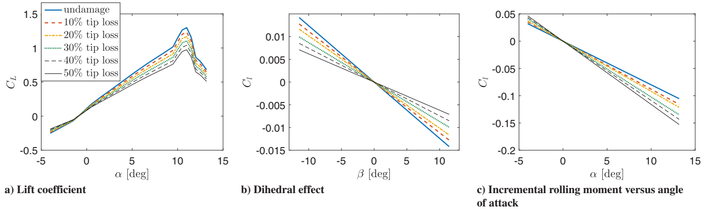
Fig. 6 Aerodynamic effects of different levels of wing damage.
