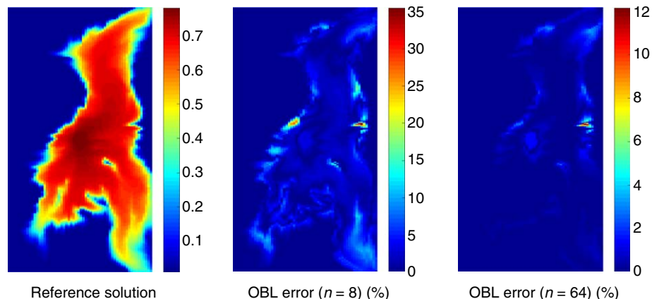
Fig. 5—Composition of \text{CO}_2 and error distribution for two OBL resolutions after 2,000 days of simulation: reference solution; OBL error ( n = 8 ) (%); OBL error ( n = 64 ) (%).
