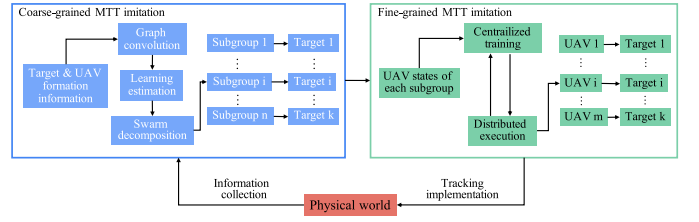
Fig. 6. Illustration of tiered DT-assisted tracking imitation.
