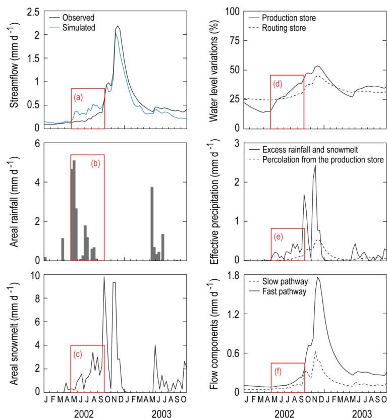
Figure 11. Internal state variables and fluxes obtained with Model C during the 2002–2003 El Niño event (using the best-performing parameter set obtained by calibration against the F_{obj} function).
