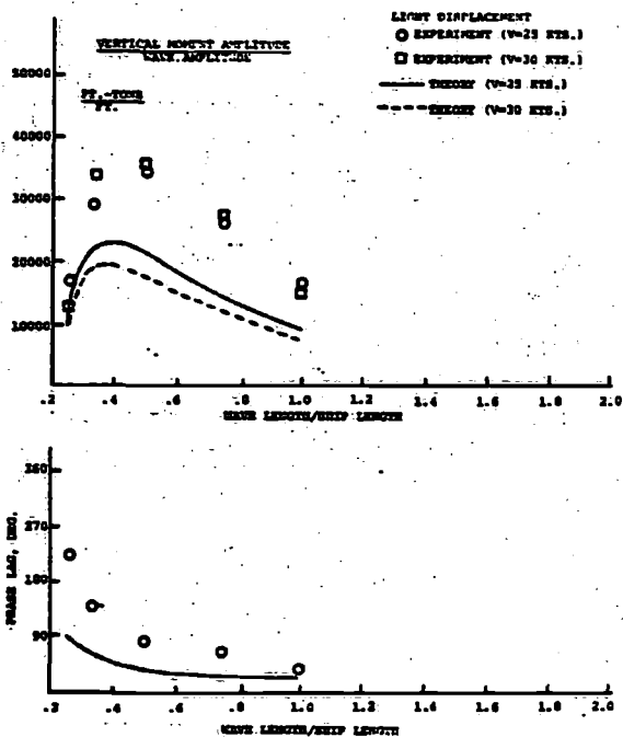
Fig. 18 - Midship Vertical Wave Bending Moments & Wave Phase Lag, 60° Heading
