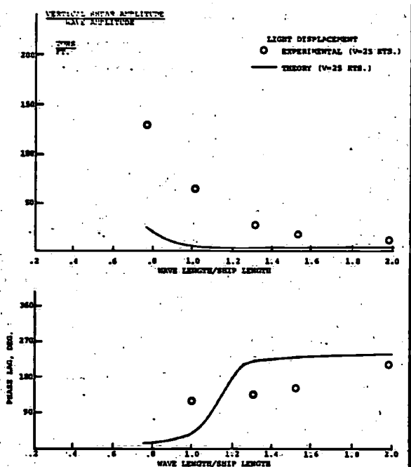
Fig. 28 - Midship Vertical Shear & Phase Lag, 0° Heading
