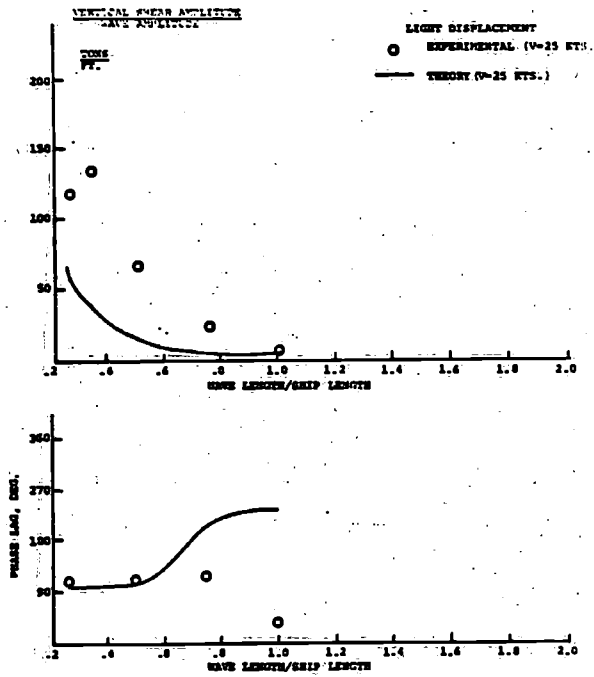
Fig. 30 - Midship Vertical Shear & Phase Lag, 60° Heading
