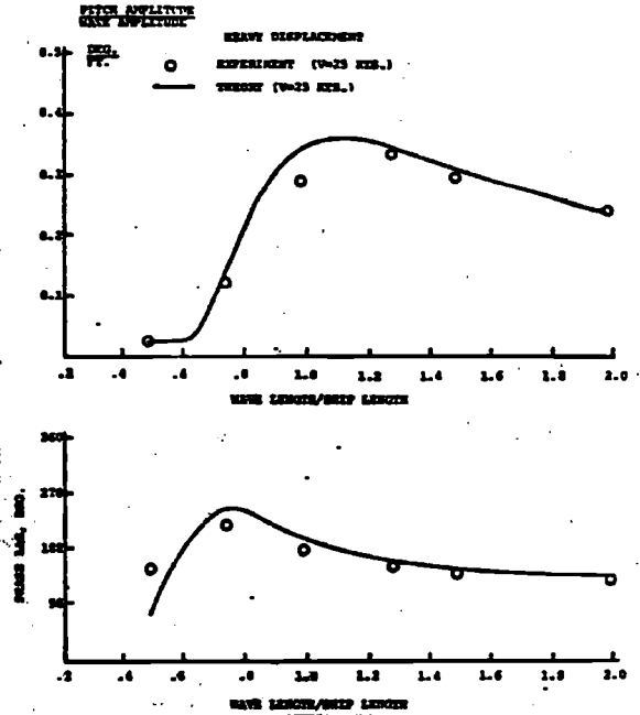
Fig. 5 - Pitch & Phase Lag, 180° Heading
