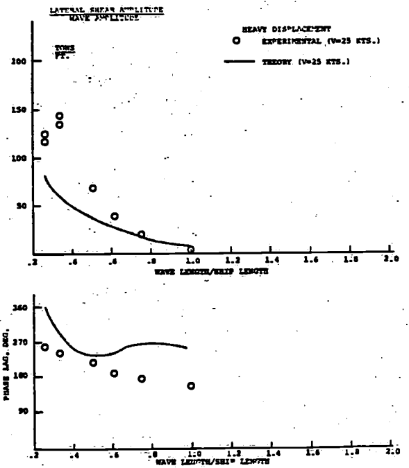
Fig. 36 - Midship Lateral Shear & Phase Lag, 240° Heading
