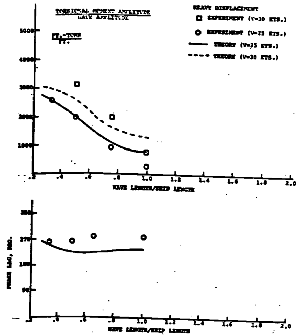
Fig. 47 - Midship Torsional Wave Bending Moments & Phase Lag, 60° Heading
