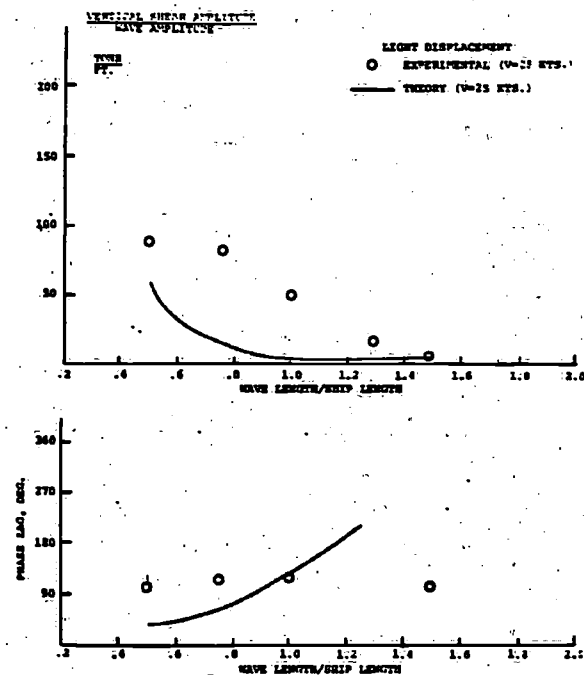
Fig. 29 - Midship Vertical Shear & Phase Lag, 30° Heading
