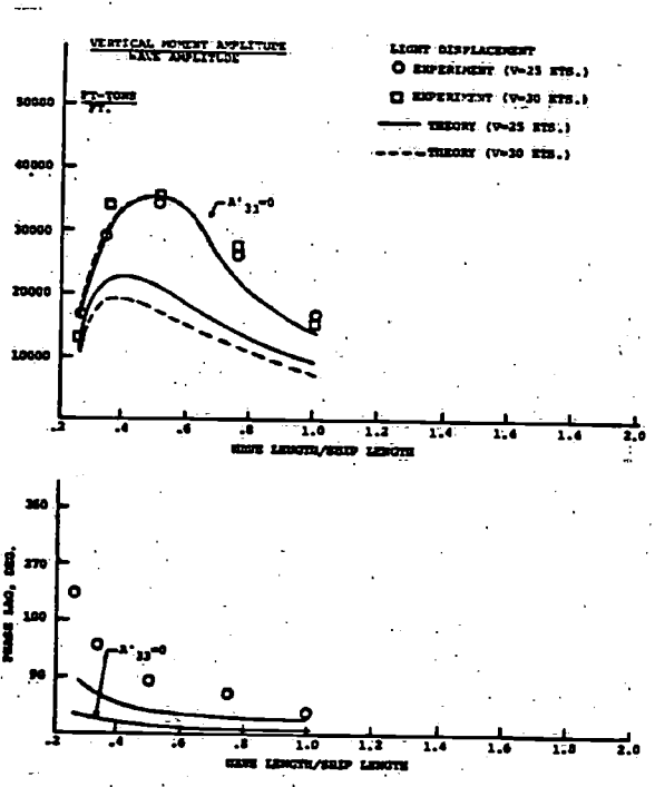
Fig. 59 - Midship Vertical Wave Bending Moments & Wave Phase Lag, 60^\circ Heading, ( A'_{33}=0 )
