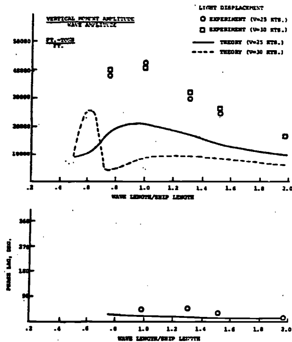
Fig. 16 - Midship Vertical Wave Bending Moments & Wave Phase Lag, 0° Heading
