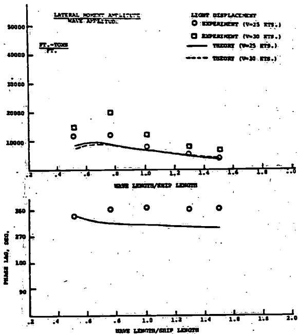
Fig. 54 - Midship Lateral Wave Bending Moments & Phase Lag, 30° Heading
