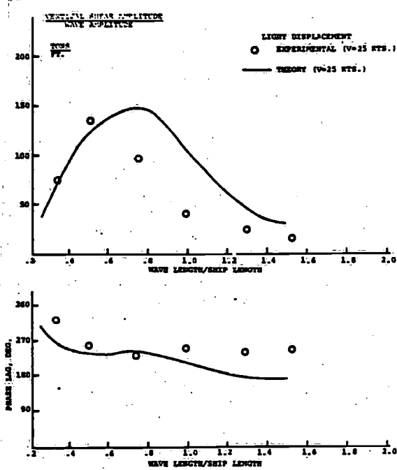
Fig. 32 - Midship Vertical Shear & Phase Lag, 210° Heading
