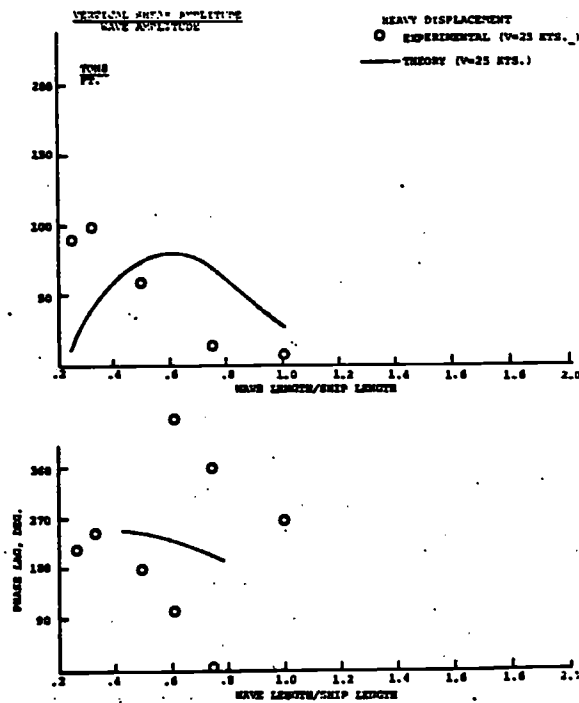
Fig. 25 - Midship Vertical Shear & Phase Lag, 240° Heading
