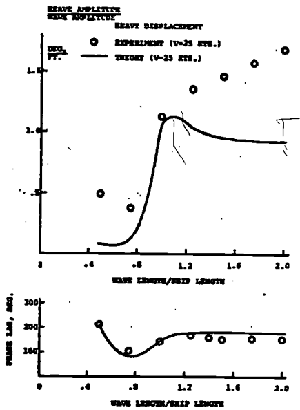
Fig. 6 - C.G. Heave & Phase Lag, 180° Heading
