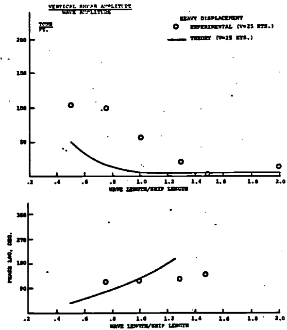
Fig. 23 - Midship Vertical Shear & Phase Lag, 30° Heading
