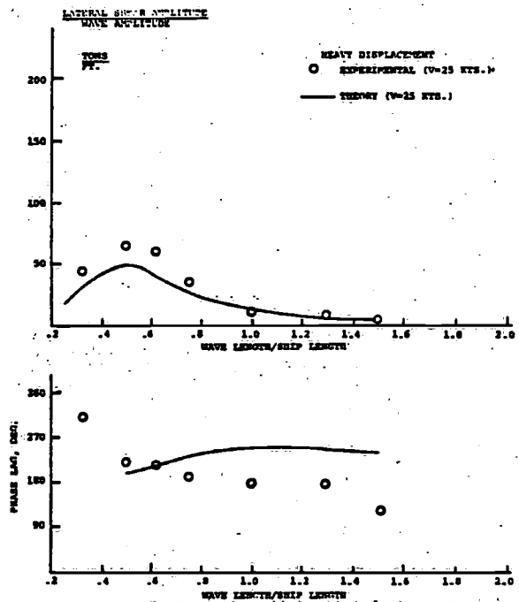
Fig. 37 - Midship Lateral Shear & Phase Lag, 210° Heading
