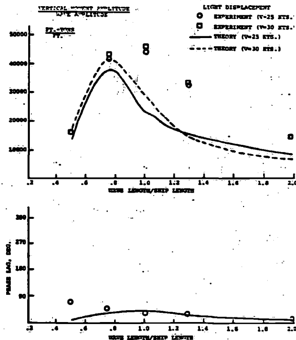
Fig. 21 - Midship Vertical Wave Bending Moments & Wave Phase Lag, 180° Heading
