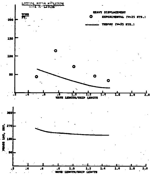
Fig. 34 - Midship Lateral Shear & Phase Lag, 30° Heading
