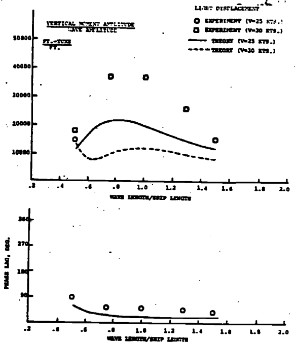
Fig. 17 - Midship Vertical Wave Bending Moments & Wave Phase Lag, 30° Heading
