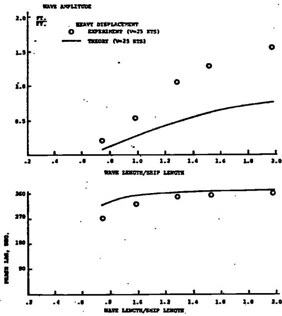
Fig. 2 - Frame 124 Heave & Phase Lag, 0° Heading
