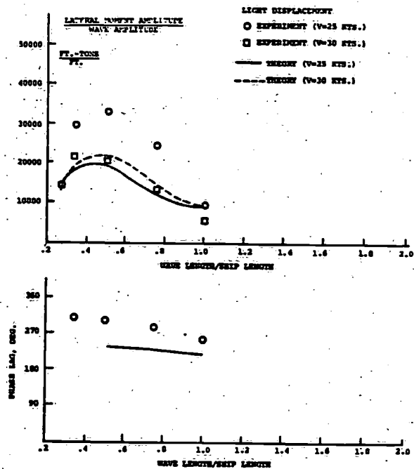
Fig. 55 - Midship Lateral Wave Bending Moments & Phase Lag, 60° Heading
