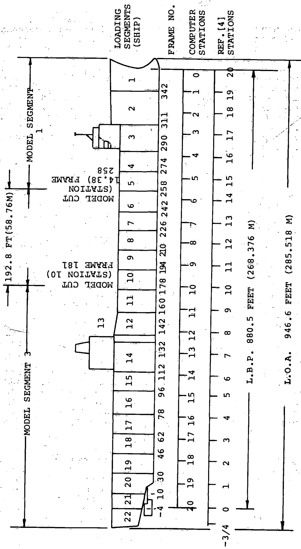
FIG. 1 LONGITUDINAL SEGMENTATION: SL-7 CONTAINERSHIP
