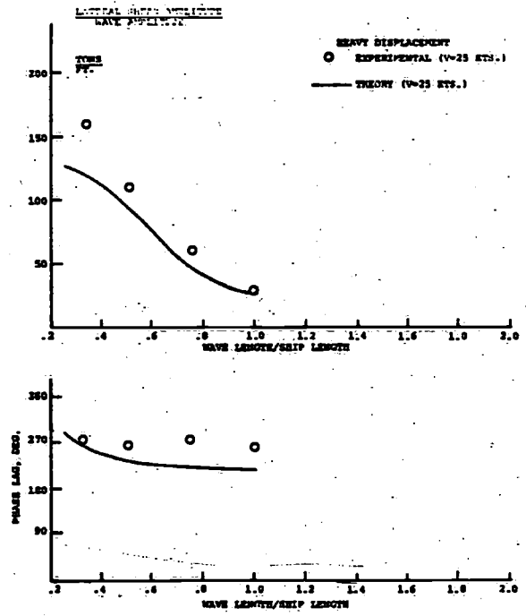
Fig. 35 - Midship Lateral Shear & Phase Lag, 60° Heading
