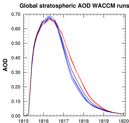
Figure 9. Global stratospheric mean AOD of the five CESM-WACCM ensemble runs. Easterly phase nudged QBO forcing is used from the observed strength starting with 1982 for two runs (red), and from the observed strength starting with 1991 for three runs (blue). The ensemble mean of the five runs is in black. Vertical dotted line marks date of injection of \text{SO}_2 .
