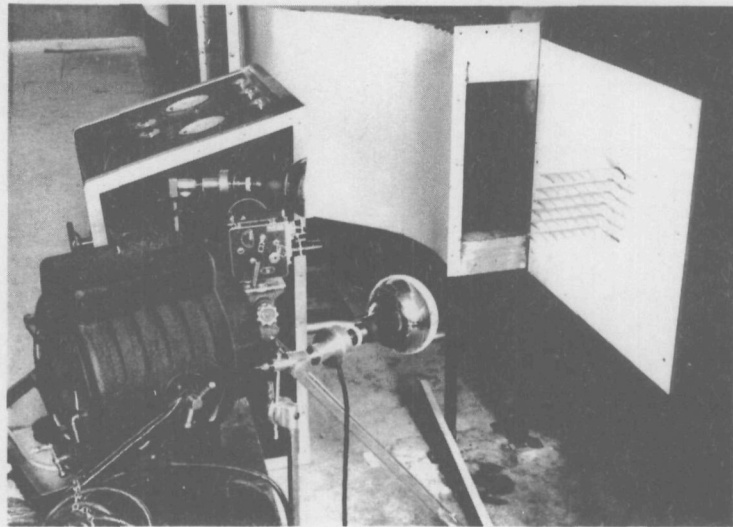
FIG. 5 ARRANGEMENT OF THE PHOTOGRAPHIC EQUIPMENT.
