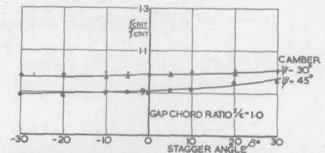
VARIATION OF CRITICAL FREQUENCY RATIO \frac{f_{CRIT}}{f_{CRIT}} WITH STAGGER ANGLE \beta
