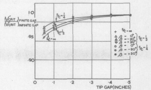
VARIATION OF CRITICAL FLUTTER SPEED RATIO WITH TIP GAP FOR VARIOUS GAP CHORD RATIOS ( \frac{3}{4} )
