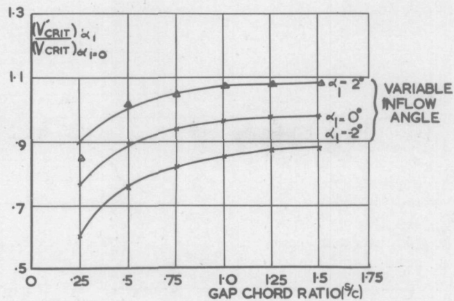
VARIATION OF \frac{(V_{CRIT})_{\alpha_1}}{(V_{CRIT})_{\alpha_1=0^\circ}} CRITICAL FLUTTER SPEED FOR CASCADE WITH GAP-CHORD RATIO CRITICAL FLUTTER SPEED FOR ISOLATED AEROFOIL AT ZERO INFLOW ANGLE (V_{CRIT})_{\alpha_1=0^\circ}
