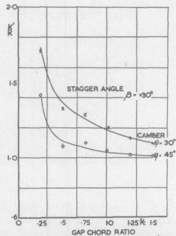
FIG7D VARIATION OF REDUCED FREQUENCY RATIO ( \frac{K'K}{K} ) WITH GAP-CHORD RATIO ( \frac{s}{c} )
