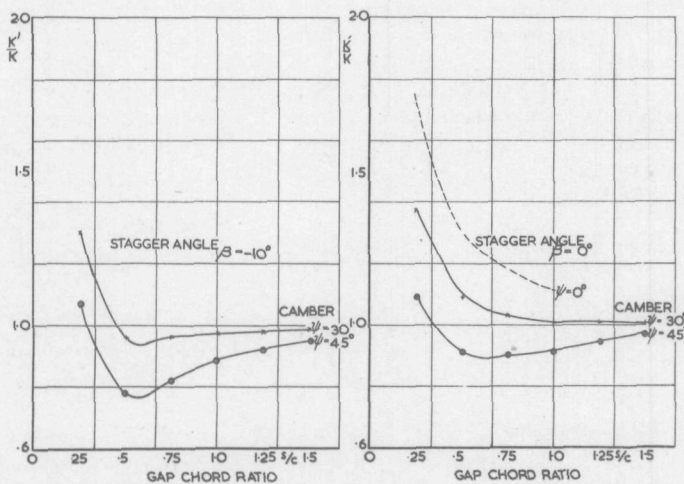
FIG7B VARIATION OF REDUCED FREQUENCY RATIO ( \frac{K'K}{K} ) WITH GAP-CHORD RATIO ( \frac{s}{c} )
