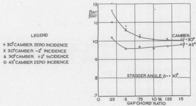
FIG.15E VARIATION OF CRITICAL FREQUENCY RATIO \frac{f_{CRIT}}{f_{CRIT}} WITH GAP CHORD RATIO \%c
