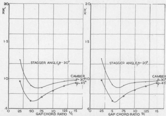
FIG7A VARIATION OF REDUCED FREQUENCY RATIO ( \frac{K'K}{K} ) WITH GAP-CHORD RATIO ( \frac{s}{c} )
