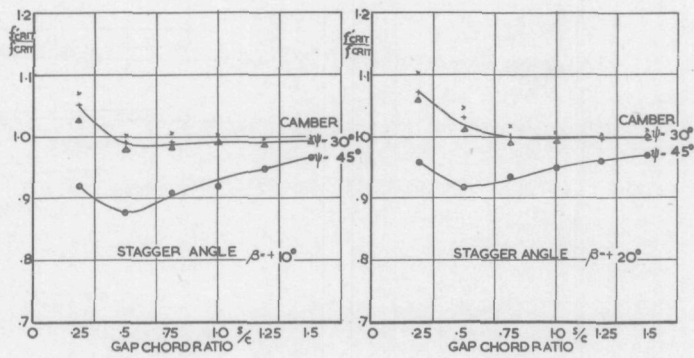
FIG.15D VARIATION OF CRITICAL FREQUENCY RATIO \frac{f_{CRIT}}{f_{CRIT}} WITH GAP CHORD RATIO \%c
