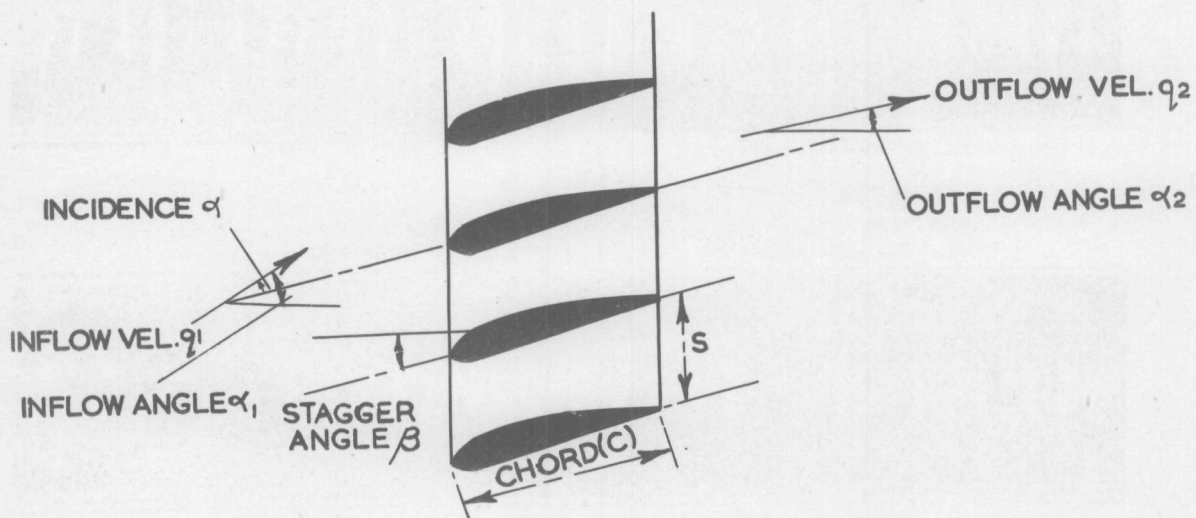
FIG.20. CASCADE GEOMETRY
