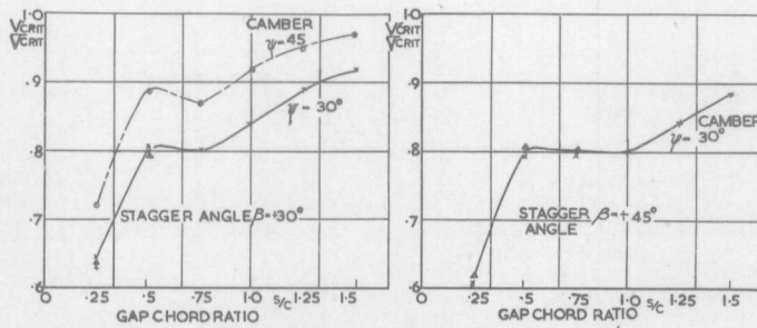
VARIATION OF CRITICAL FLUTTER SPEED RATIO \frac{V_{CRIT}}{V_{CRIT}} FIG 13 E WITH GAP CHORD RATIO s/c .
