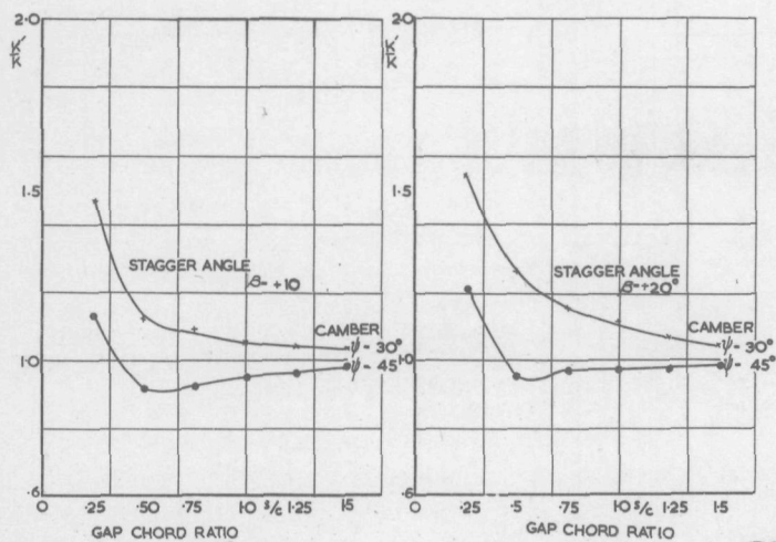
FIG7C VARIATION OF REDUCED FREQUENCY RATIO ( \frac{K'K}{K} ) WITH GAP-CHORD RATIO ( \frac{s}{c} )
