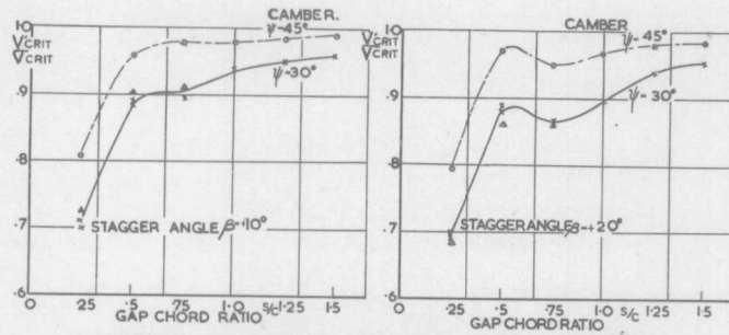
VARIATION OF CRITICAL FLUTTER SPEED RATIO \frac{V_{CRIT}}{V_{CRIT}} FIG 13 D. WITH GAP CHORD RATIO s/c .
