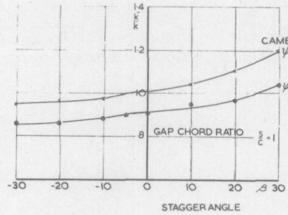
VARIATION OF REDUCED FREQUENCY RATIO ( K_k ) WITH STAGGER ANGLE ( \beta^\circ )
