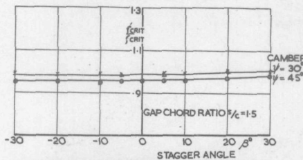
VARIATION OF CRITICAL FREQUENCY RATIO \frac{f_{CRIT}}{f_{CRIT}} WITH STAGGER ANGLE \beta
