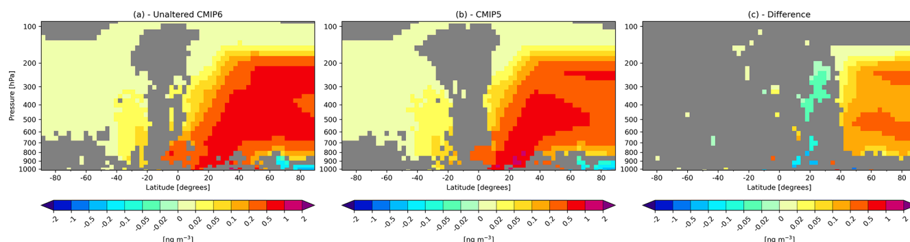
Figure 3. Zonally averaged aviation-induced changes in black carbon concentration simulated by the model using the unaltered CMIP6 (a) and CMIP5 (b) inventory and their difference (c). Gray areas mark non-significant changes at the 95 % confidence level.
