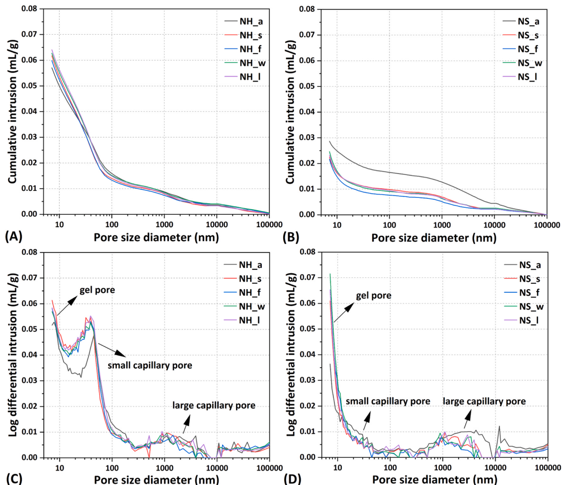
Fig. 7. Cumulative intrusion and log differential intrusion of 28 d AASM cured under five conditions ranging from 7 nm to 100 \mu\text{m} .
