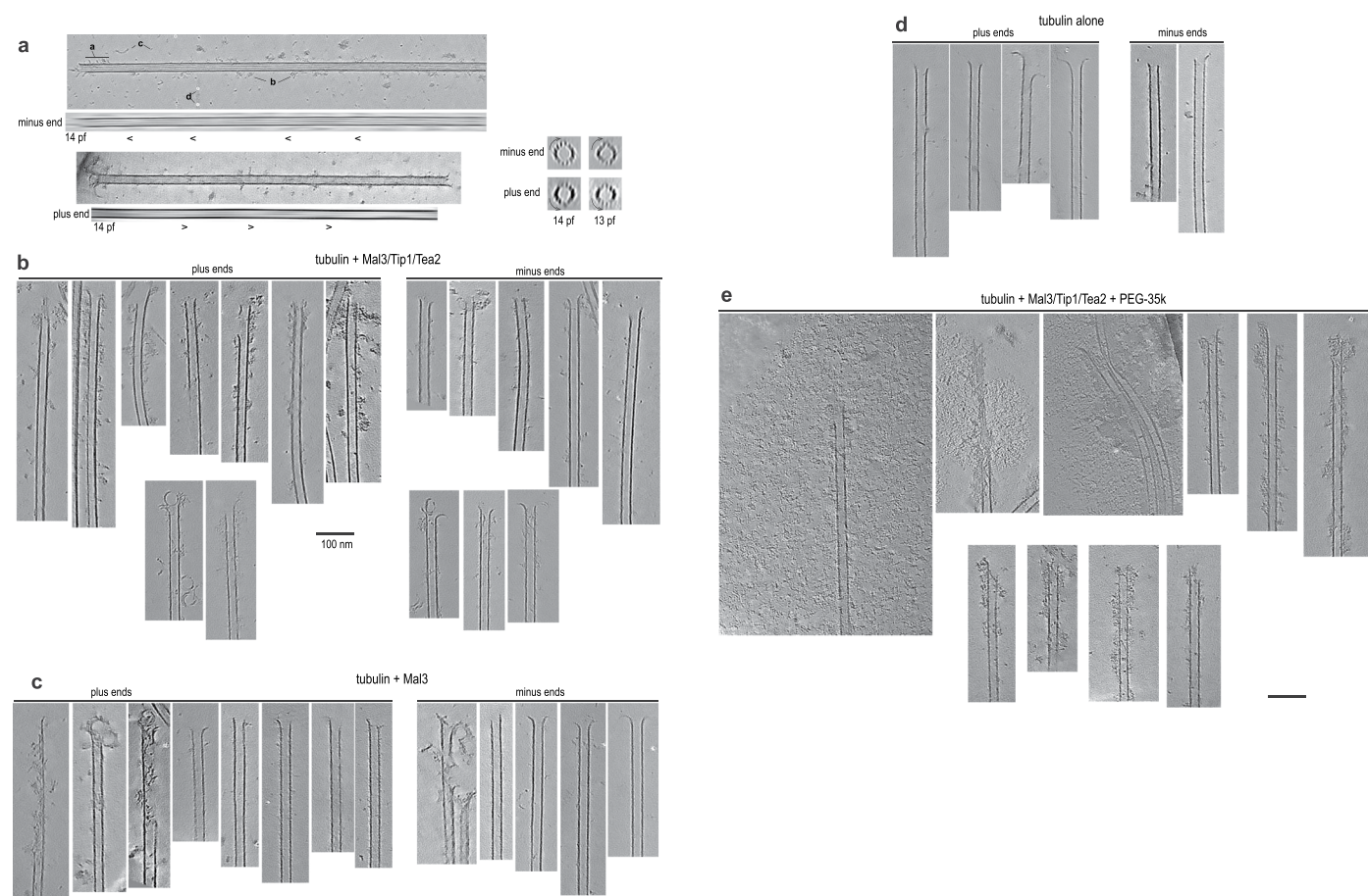
Extended Data Fig. 3 | (a) Summed tomogram slices containing microtubules (top) and Fourier-filtered subsets containing microtubule moiré pattern (bottom). Two examples are shown: a 14-protofilament microtubule with the minus end pointing up, and a 14-protofilament microtubule with the plus-end pointing up. a – comet at the minus-end, b – Mal3/Tip1/Tea2 oligomers bound to microtubule lattice, c – soluble tubulin oligomers, d – gold particles with
