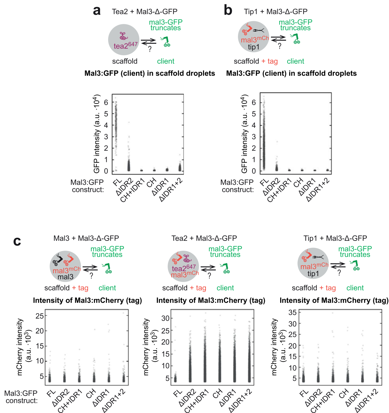
Extended Data Fig. 5 | (a) Droplets of Tea2-647 (scaffold) were allowed to recruit Mal3:GFP constructs (2 nM, client) in the presence of PEG-6k. The graph shows distribution of Mal3:GFP construct intensity in the scaffold droplets (number of droplets n = 358, 4178, 5220, 6023, 5317, 6065 ; from left to right). (b) Droplets of unlabelled Tip1 (scaffold) tagged with FL-Mal3:mCherry (2 nM, tag) were allowed to recruit Mal3:GFP constructs (2 nM, client) in presence of
