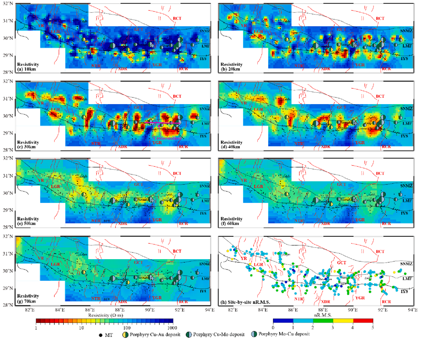
Fig. 7. 3-D electrical resistivity model. (a)–(g) Horizontal slices of the electrical resistivity. Labels as in Fig. 1. (h) Site-by-site nR.M.S. misfit of the 3-D inversion. Pink line in 7c is shown in Fig. 6a. Refer to Fig. 1 for labels. (For interpretation of the references to colour in this figure legend, the reader is referred to the web version of this article.)
