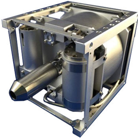
Figure 18.7 The BGT-X5 mono-propellant system from Busek [7].
