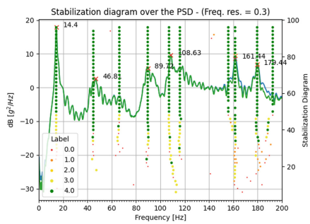
Fig. 16. Damage level 3 PCB equipment, results in frequency spectrum
