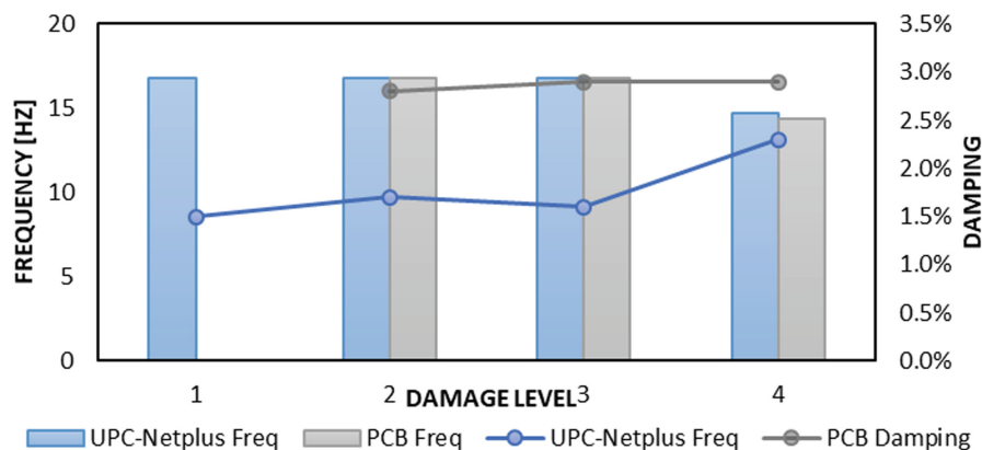
Fig. 17. Frequency and damping with different damage levels
