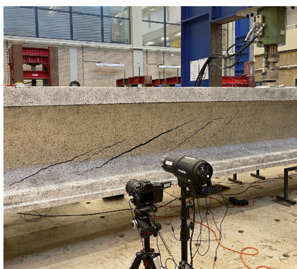
Fig. 6. Damage level 3. Failure
