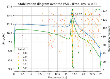
Fig. 11. Damage level 1 UPC-Netplus equipment, results in frequency spectrum
