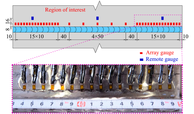
Fig. 2. Strain gauges installed at the region of interest.
