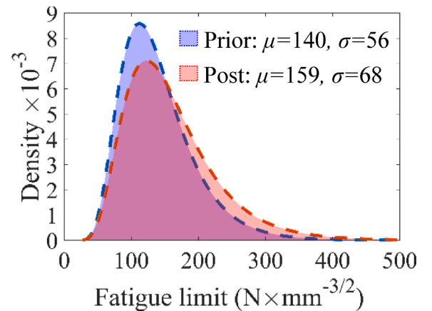
Fig. 21. Prior and posterior distribution of fatigue limit in specimen T7.
