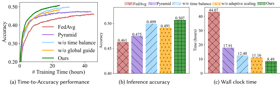
Fig. 9. The ablation study of ShuffleFL on the Shakespeare dataset. Wall clock time indicates the time consumption when reaching the target accuracy.
