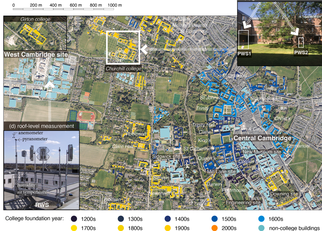
Fig. 2. Map showing: (a) & (b) locations of East Anglia and the city of Cambridge; (c) all courtyard locations and the foundation years of corresponding colleges/teaching sites in Cambridge; (d) the RWS location at Computer Laboratory in West Cam site; (e) the validation courtyard in Churchill College, with the two PWSs highlighted.
