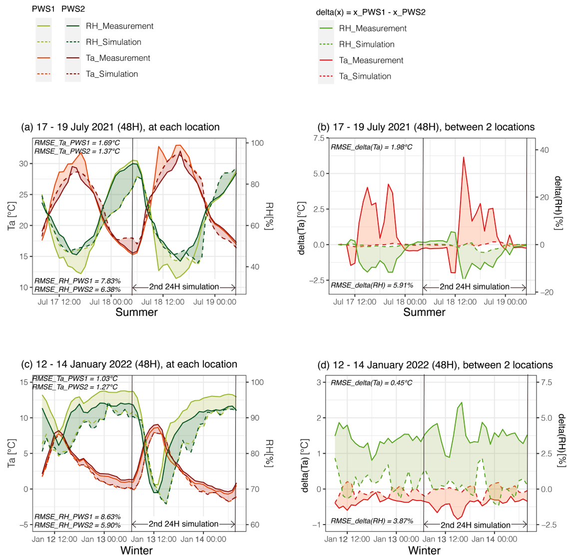
Fig. B.1. The RMSE results of T_a , RH, \Delta(T_a) , and \Delta(RH) between ENVI-met and 2 PWSs in the courtyard in Churchill College.
