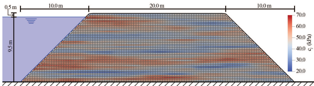
Figure 1. Problem description of MPM dyke simulation highlighting a single random field of initial undrained shear strength c_i . The random field uses \theta_v = 1.0 m and \theta_h = 24 m.
