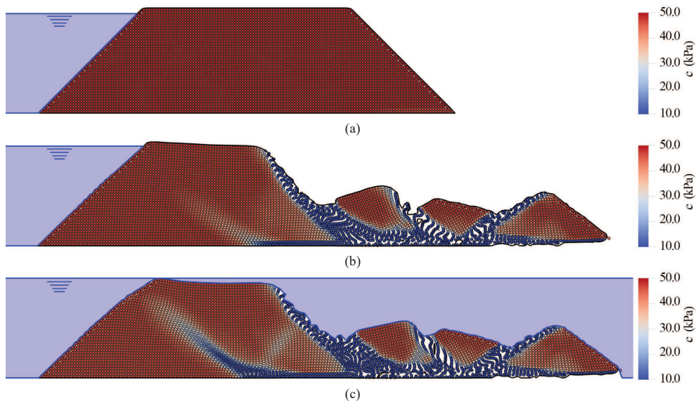
Figure 2. Rotational slope failure mechanisms for homogeneous dykes with slightly different initial cohesion: (a) no failure for c_i = 48 kPa; (b) initial slope failure for c_i = 47 kPa; (c) flooding for c_i = 46 kPa.
