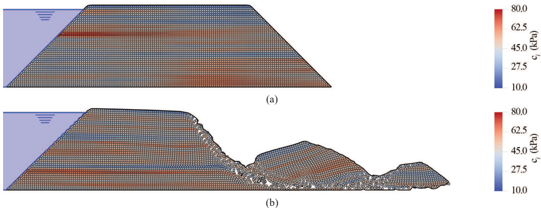
Figure 4. Realizations without ULS dyke failure for random fields with \theta_h = 48 m: (a) no initial slope failure; (b) initial failure with enough residual dyke strength to prevent ULS failure.
