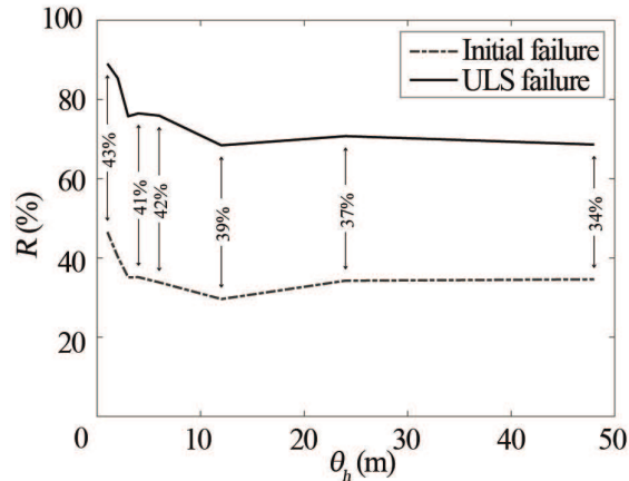
Figure 7. Effect of horizontal scale of fluctuation on initial and ULS reliability at end of simulations.
