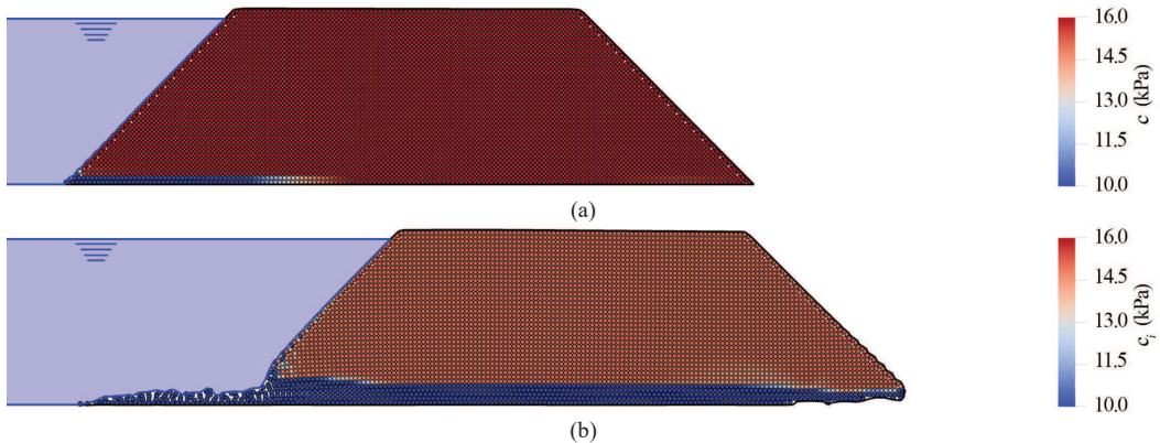
Figure 3. Horizontal dyke failure mechanisms for homogeneous dykes with slightly varying initial cohesion: (a) no failure for c_i = 16 kPa; (b) complete failure for c_i = 15 kPa.
