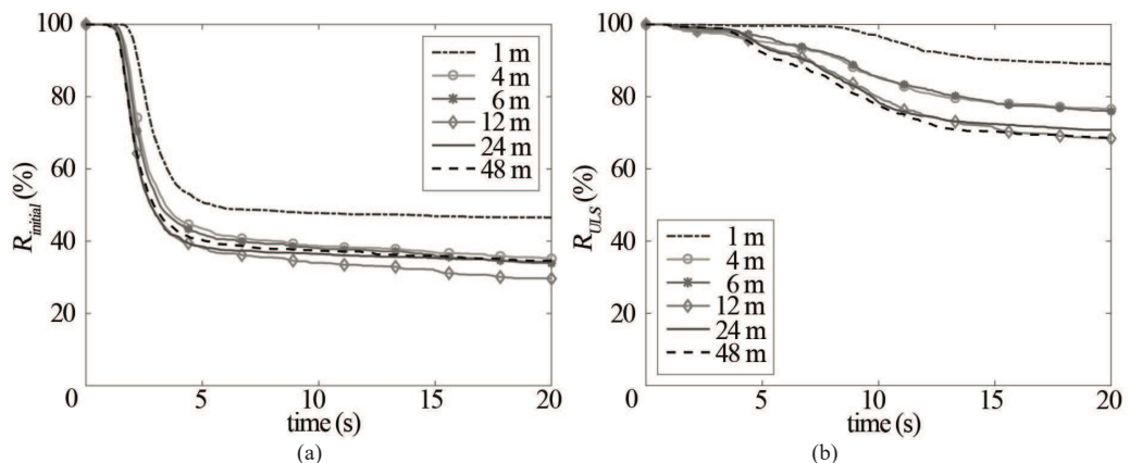
Figure 6. Development of reliability over time: (a) reliability against initial failure (without residual dyke strength); (b) reliability against ULS failure (with residual dyke strength).
