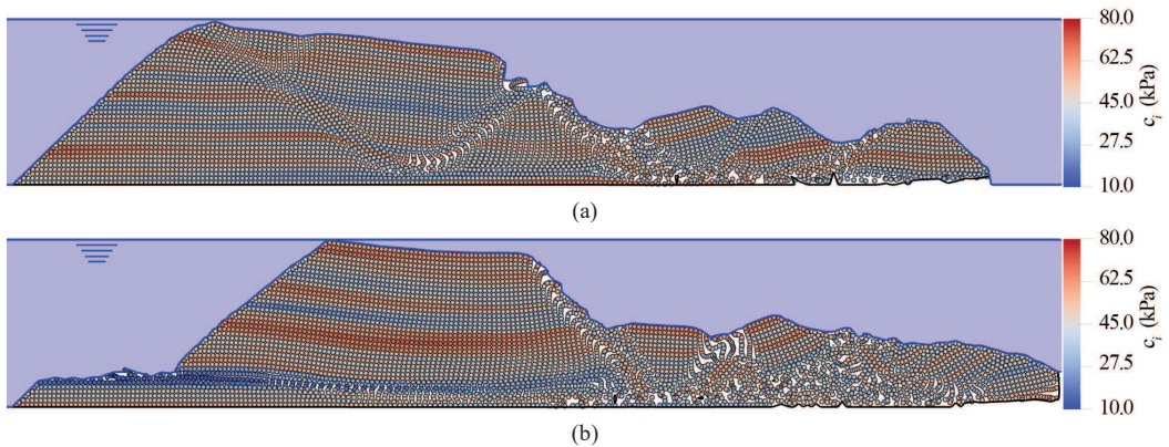
Figure 5. Realizations with ULS dyke failure for random fields with \theta_h = 48 m: (a) rotational retrogressive failure; (b) initial slope failure followed by a horizontal slide through a weak layer.
