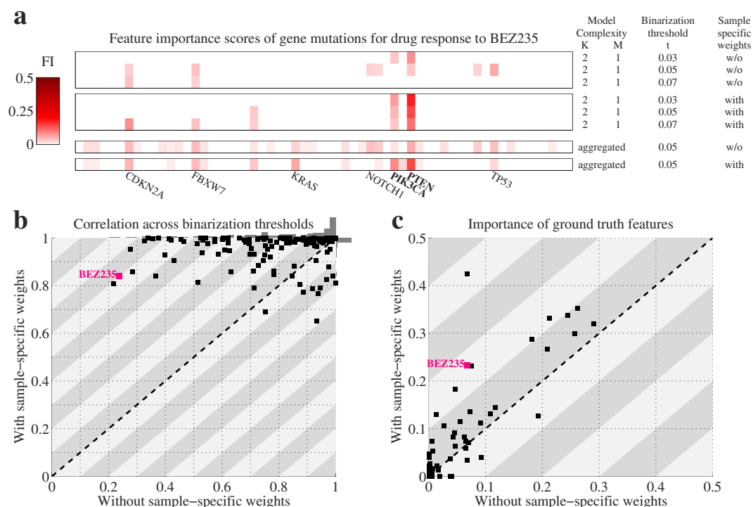
Figure 3. LOBICO's use of continuous output leads to robust and accurate models. (a) Heatmaps depicting the feature importance (FI) scores across the 60 gene mutations for the logic models inferred to explain the drug response to the PI3K/mTOR inhibitor BEZ235. The upper heatmap represents FI scores for the 2-input OR model ( K=2 , M=1 ) using three different binarization thresholds for logic models with binarized output, i.e. not using the sample-specific weights. The middle of the three heatmaps represents the same FI scores, but for logic models with continuous output, i.e. using the sample-specific weights. The bottom two heatmaps depict FI scores aggregated across all model complexities, using the standard binarization threshold ( t=0.05 ), for both the logic models with and without the sample-specific weights. The labels of the gene mutations with a large FI in any of these heatmaps are printed below. The 'ground truth' features, i.e. the expected or annotated targets of this drug, PTEN and PIK3CA, are printed in bold. (b) Scatter plot with the average Pearson correlation coefficients of the similarity of FI scores across the binarization thresholds for inferred logic models without (x-axis) and with (y-axis) the sample-specific weights. Each point represents one of the 142 drugs. The correlation scores are computed using the model-complexity-specific FI scores. The grey bars on top and to the right of the scatter plot represent histograms of these correlation scores for models without and with the sample-specific weights, respectively. (c) Scatter plot with the importance of the ground truth features for inferred logic models without (x-axis) and with (y-axis) the sample-specific weights. Each point represents one of the 49 drugs, for which ground truth features were available. The importance scores of the ground truth features were derived from aggregated FI scores.
