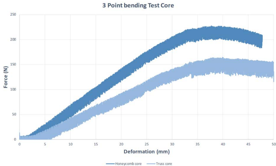
Diagram 01: Result 3 – point bending test core element.
