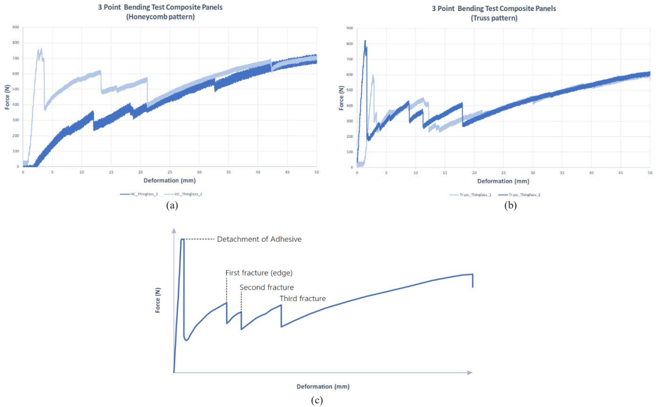
Diagram 2a) Result of 3 PBT unaffected composite panel with honeycomb pattern, b) Result of 3 PBT unaffected composite panel with truss pattern, c) structural behavior of the composite panel unaffected.
