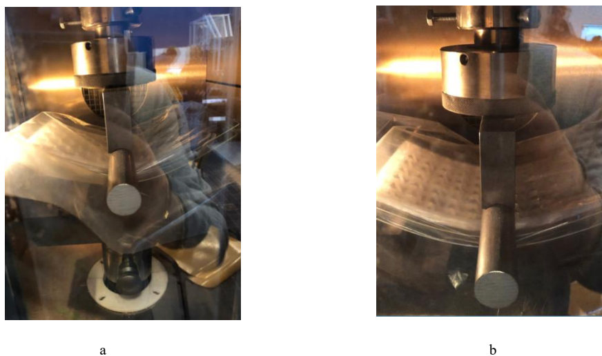
Fig. 13a) Composite panel (honeycomb core) with a deflection of 50mm at 80 °C, b) Composite panel (truss core) with a deflection of 50mm at 80 °C.
