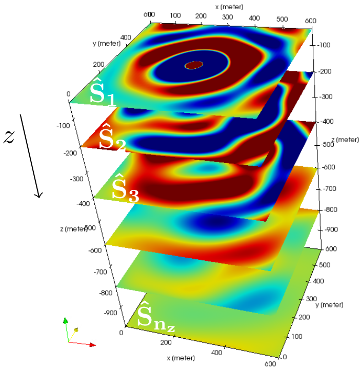
Figure 4.7: Schematic illustration: The diagonal blocks of \hat{S} in (4.24) correspond to a sequence of n_z 2D problems in the xy -plane.
