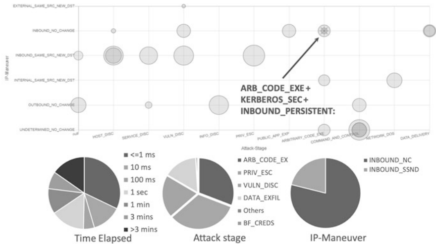
Fig. 6.5 (Top) A screenshot of attack models produced by ASSERT with a persistent arbitrary code execution through Kerberos. (Bottom) The pie charts show the model’s attack features in Attack Speed, Attack Intent Stage, and Attack Maneuver. (Adapted from Yang et al., 2021)
