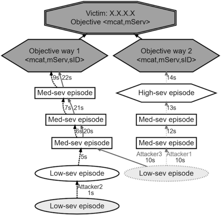
Fig. 6.8 A notional alert-driven attack graph showing paths towards an objective. Each vertex represents an episode. The vertex labels are <mcats, mServ, sID>, reflecting the AIF attack stage, targeted service, and state identifier from S-PDFA. The vertex shape indicates the episode severity. The root nodes reflect the attacker’s objective and the victim host. The dotted vertices reflect the sink states. The edges show attack progression and are annotated with the time since the first alert was captured. The attacker’s IP address is stated next to the first action in an attack path. (Adapted from Nadeem et al., 2021c)
