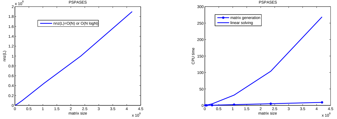
Figure 3: Complexity of PSPASES; memory requirements (left) and CPU time (right). Variable matrix order N , variance \sigma = 1 , number of processors P = 2 .
