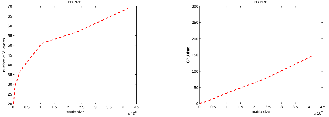
Figure 4: Complexity of HYPRE/SMG; convergence (left) and CPU time (right). Variable matrix order N , variance \sigma = 1 , number of processors P = 2 .
