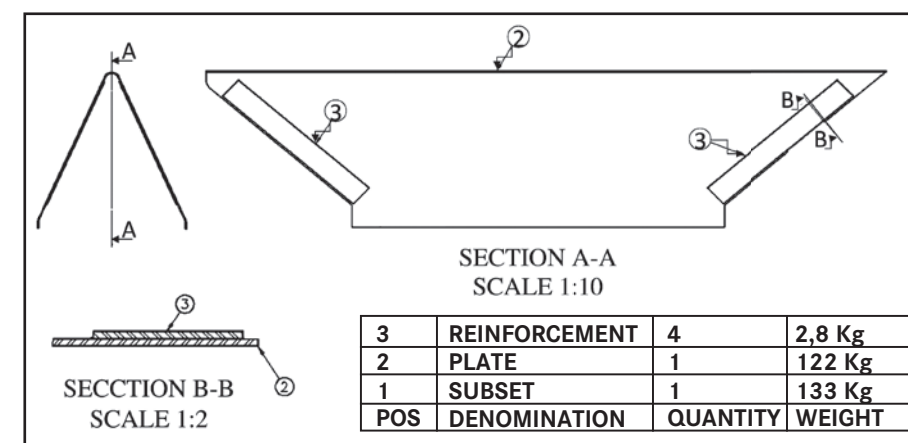
Fig. 1. Technical drawing of the subset.
